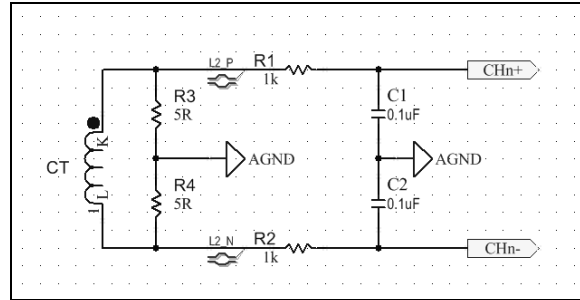
FIGURE 7-6: First-Order Anti-Aliasing Filter for CT-Based Designs.
