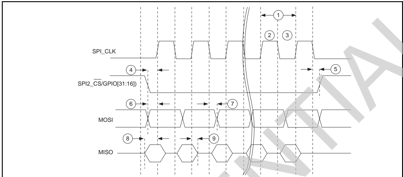
Figure 24 - SPI Timing Waveforms
