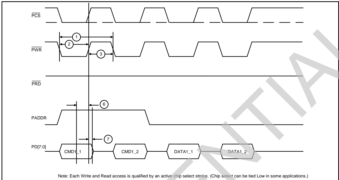
Figure 10 - GPI 8-Bit Write Access Using Separate Read and Write Strokes
