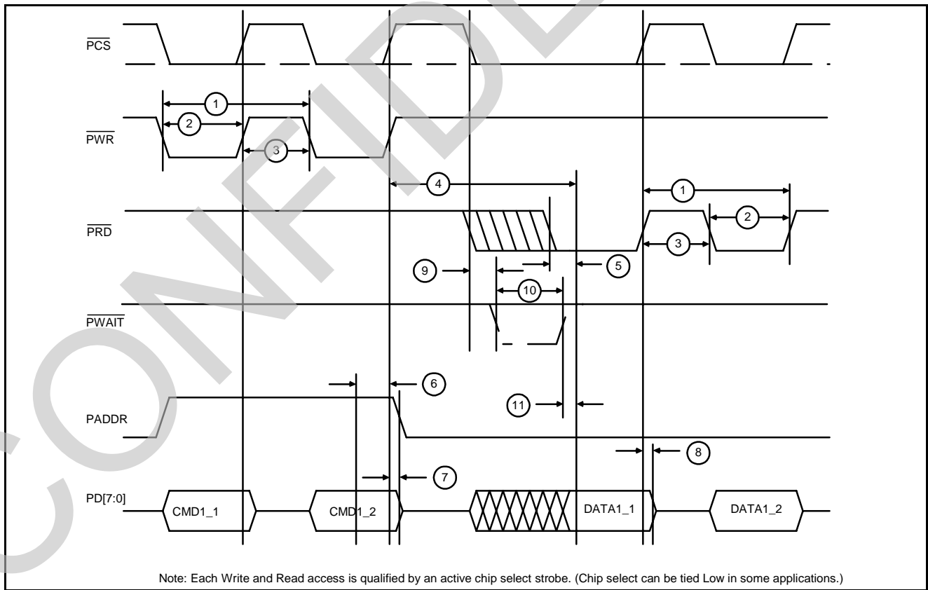
Figure 11 - GPI 8-Bit Read Access Using Separate Read and Write Strokes
