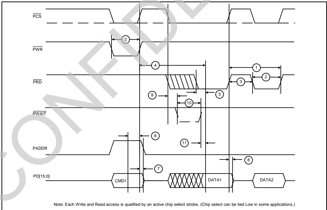
Figure 9 - GPI 16-Bit Read Access Using Separate Read and Write Strokes
