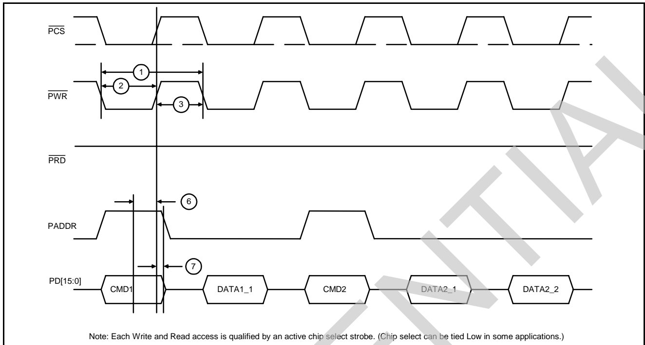
Figure 8 - GPI 16-Bit Write Access Using Separate Read and Write Strokes
