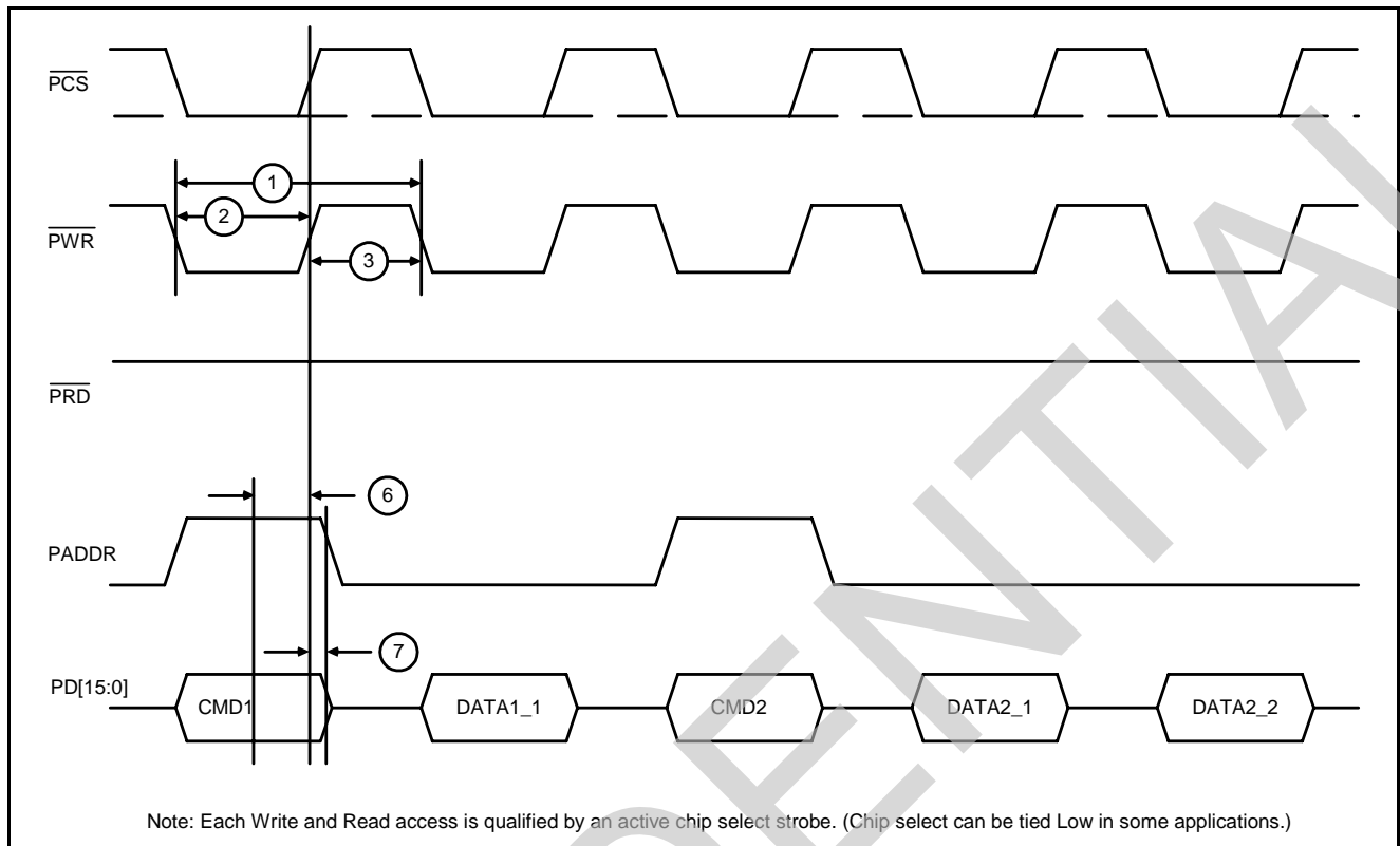
Figure 8 - GPI 16-Bit Write Access Using Separate Read and Write Strokes
