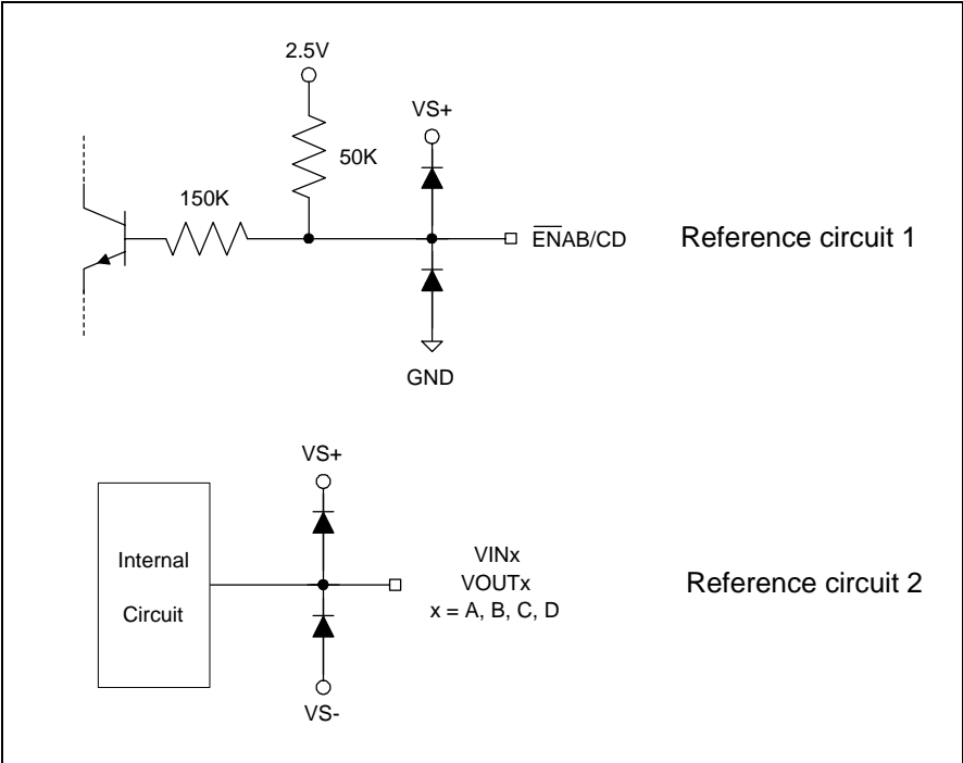
Figure 2 - Reference Circuit
