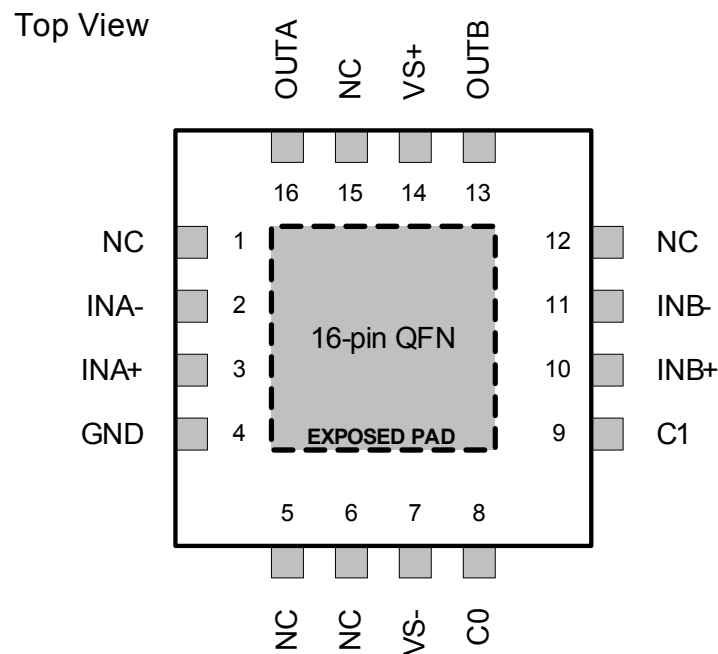
Figure 5 • Connection Diagram
