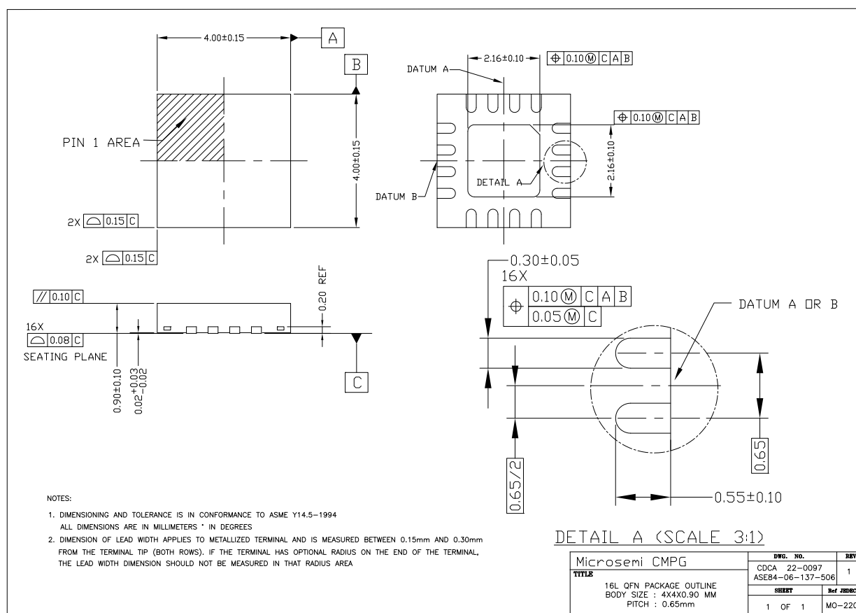
Figure 6 • Package Drawing
