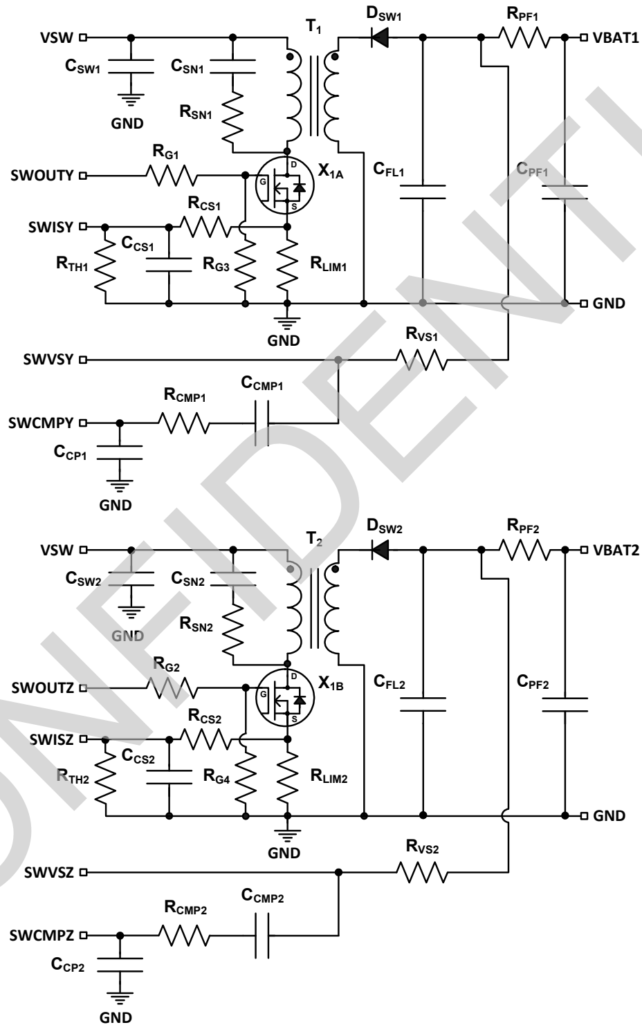
Flyback Switcher Circuit 140-V PK (Tracking) Ringing with 5 REN Load (VSW = 9 - 16V)
