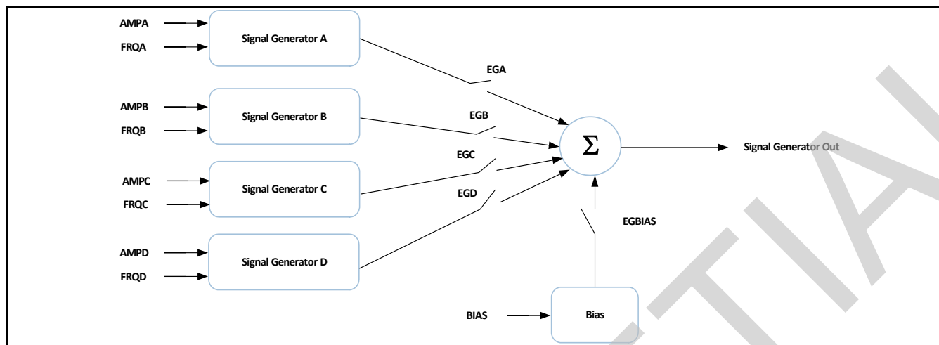
Figure 12 - Multi-Tone Generation
