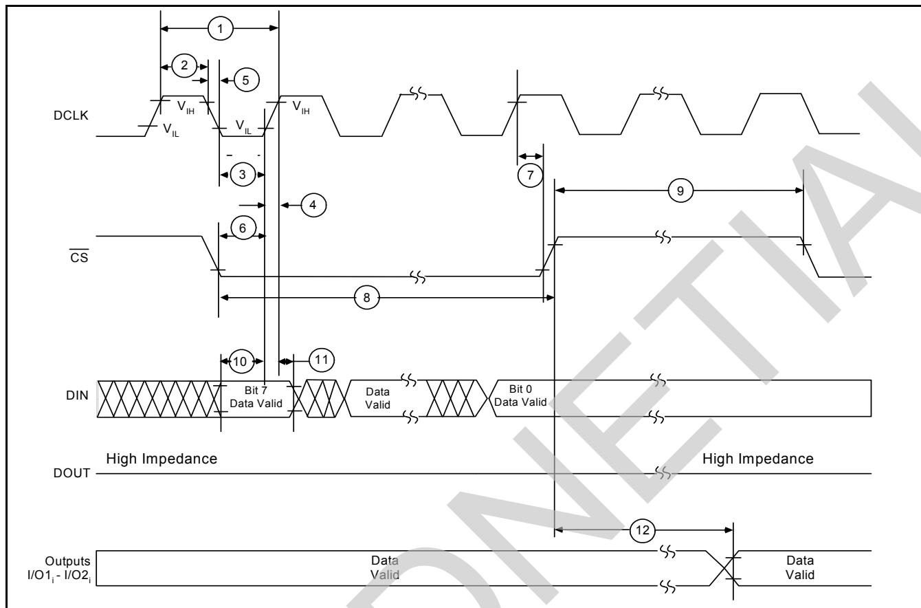
Figure 30 - SPI Interface (Input Mode)
