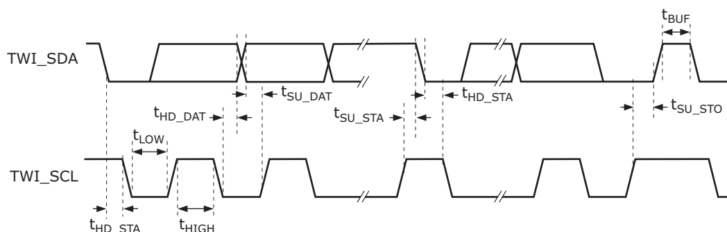
Figure 179 • Two-Wire Serial Write Timing Diagram
