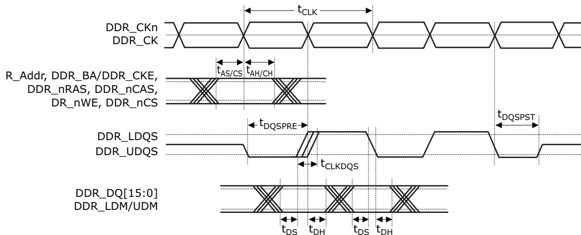
Figure 172 • DDR SDRAM Output Timing Diagram
