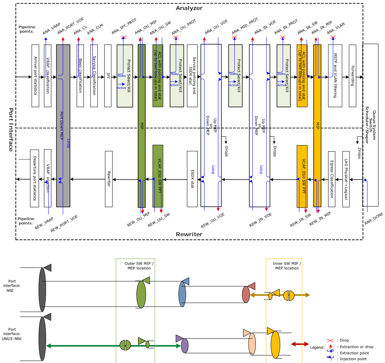
Figure 21 • Processing Flow
