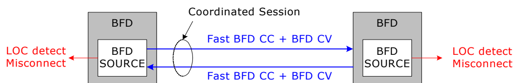
Figure 78 • BFD Coordinated Mode
