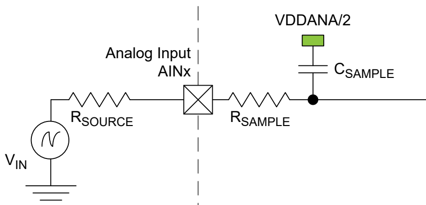
Figure 38-3. ADC Input
