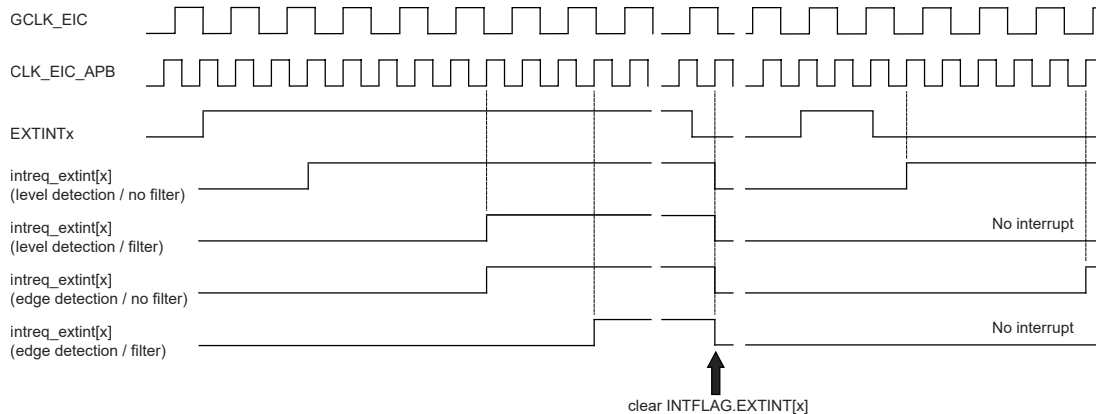
Figure 21-2. Interrupt Detections
