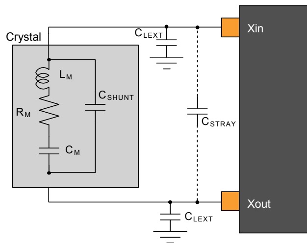
Figure 44-4. Oscillator Connection
