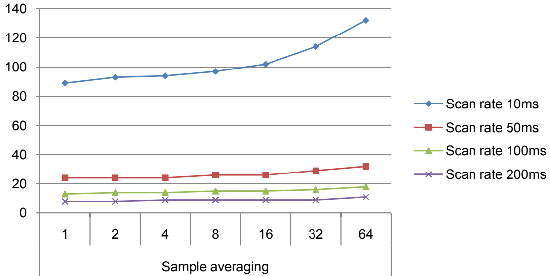
Figure 37-8. Power Consumption [ \mu A]
