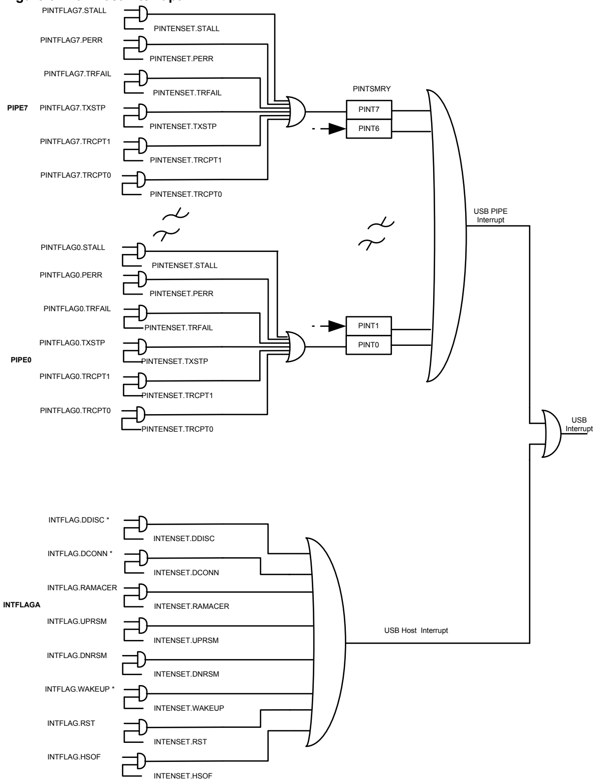
Figure 32-10. Host Interrupt
