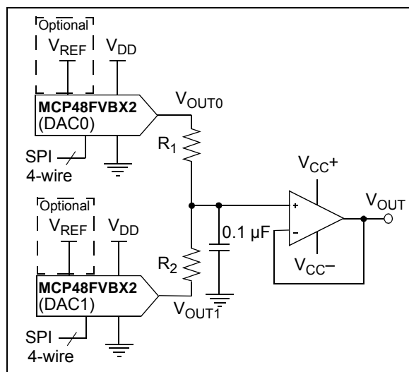
FIGURE 8-6: Simple Double-Precision DAC using MCP48FVBX2.
