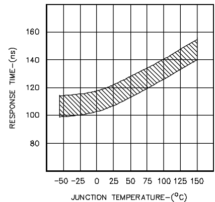
FIGURE 18. SHUTDOWN INPUT TO DRIVER OUTPUT DELAY
