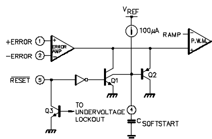
FIGURE 22. SOFT-START CIRCUIT SCHEMATIC
