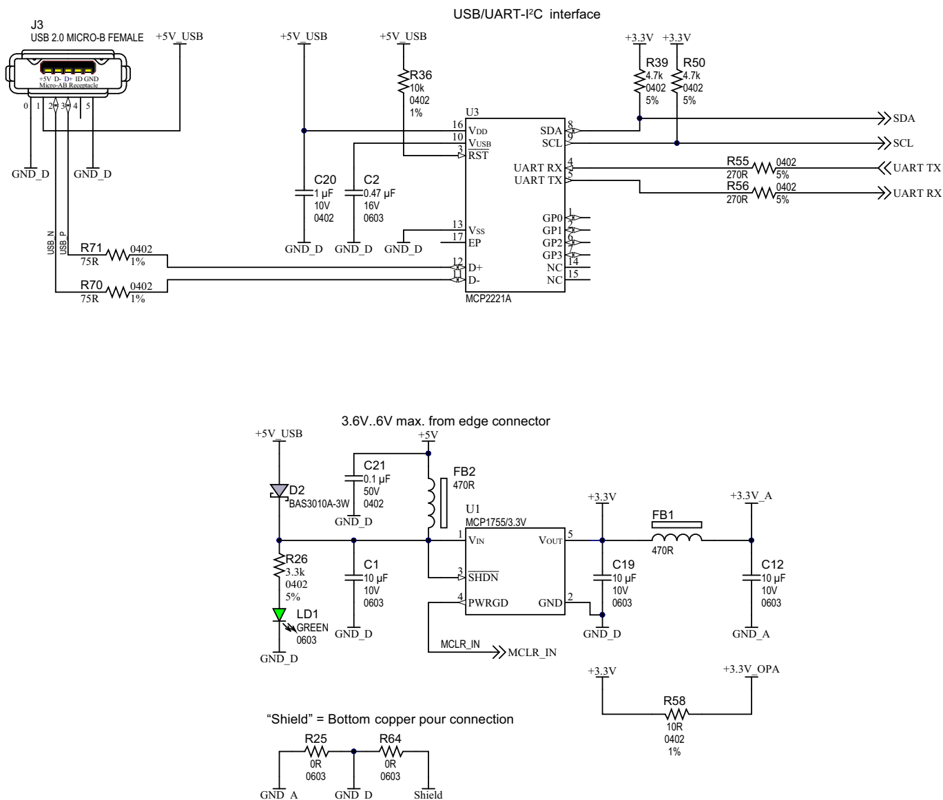
FIGURE A-2: dsPIC33EP128GS806 DIGITAL POWER PIM SCHEMATIC REV. 1.1 (PAGE 2 OF 2)
