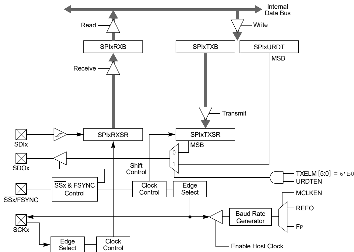
Figure 17-1. SPIx Module Block Diagram (Standard Mode)
