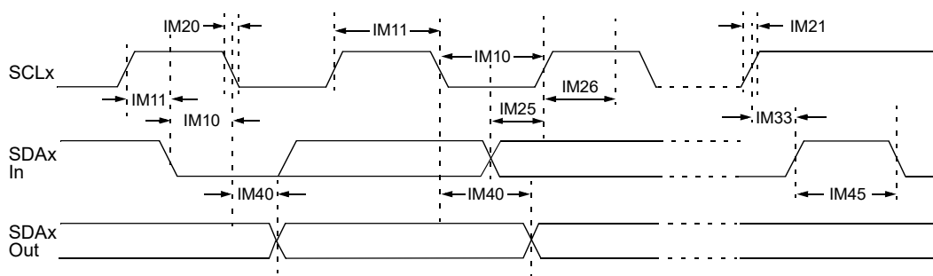
Figure 33-14. I2Cx Bus Data Timing Characteristics (Host Mode)
