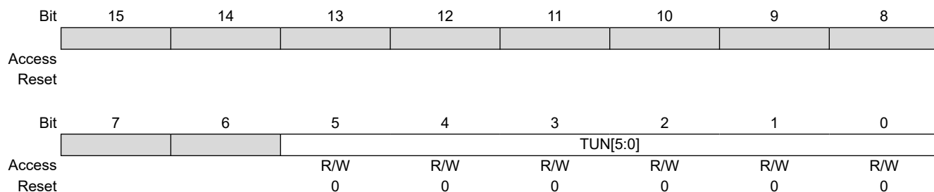
Bits 5:0 – TUN[5:0] FRC Oscillator Tuning bits
