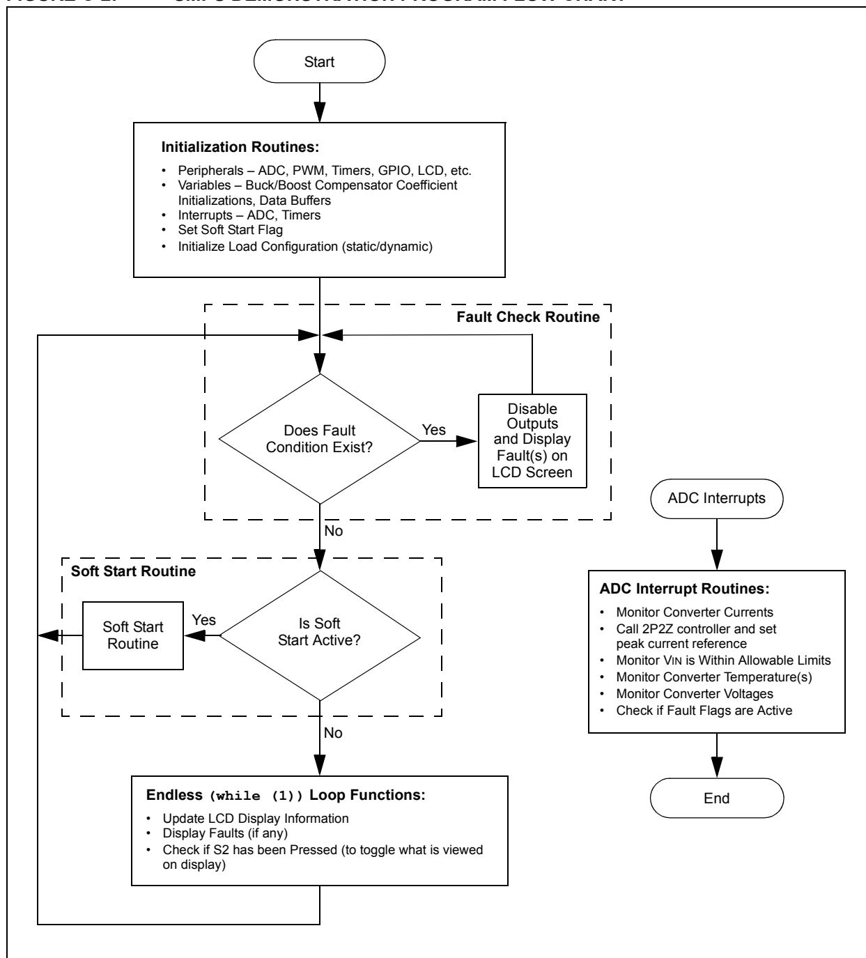
FIGURE C-2: SMPS DEMONSTRATION PROGRAM FLOW CHART
