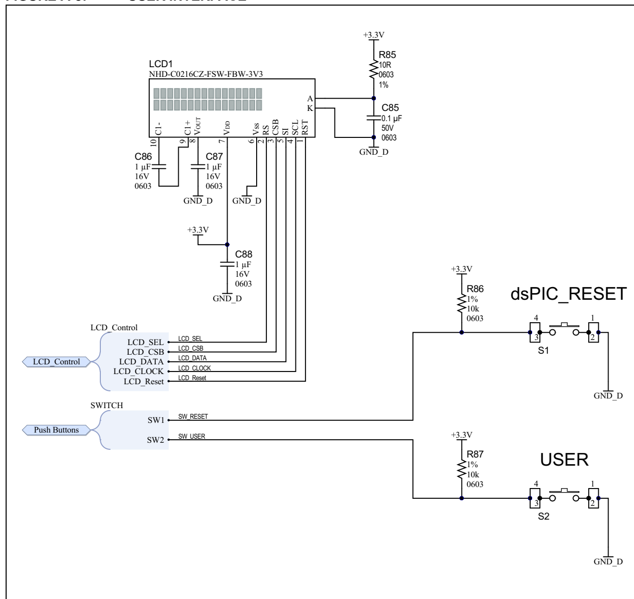
FIGURE A-8: USER INTERFACE
