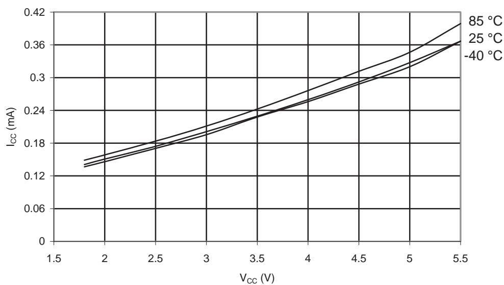
Figure 27-9. ATmega1284P: Idle Supply Current vs. V_{CC} (Internal RC Oscillator, 1 MHz)
