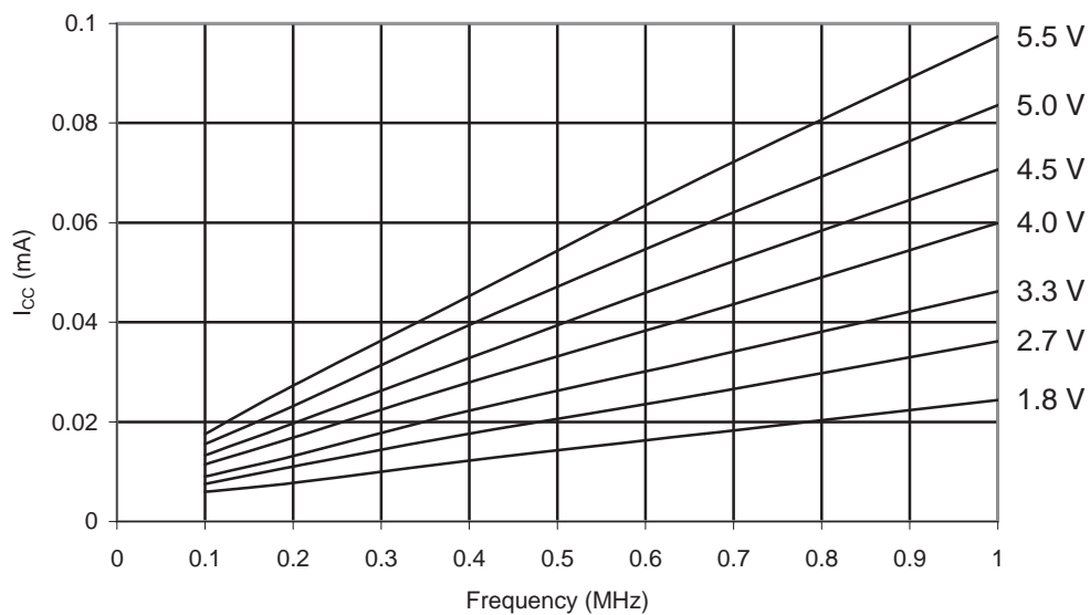
Figure 27-46. ATmega1284P: Reset Supply Current vs. Low Frequency (0.1 - 1.0 MHz)
