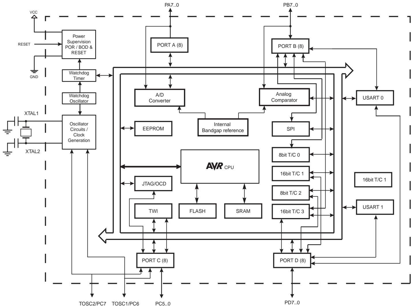
Figure 2-1. Block Diagram
