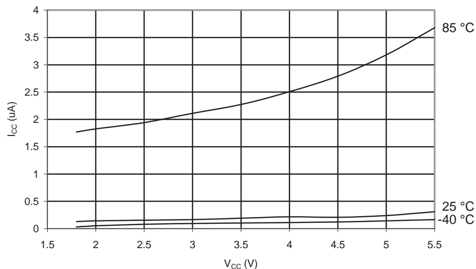
Figure 27-11. ATmega1284P: Power-down Supply Current vs. V_{CC} (Watchdog Timer Disabled)
