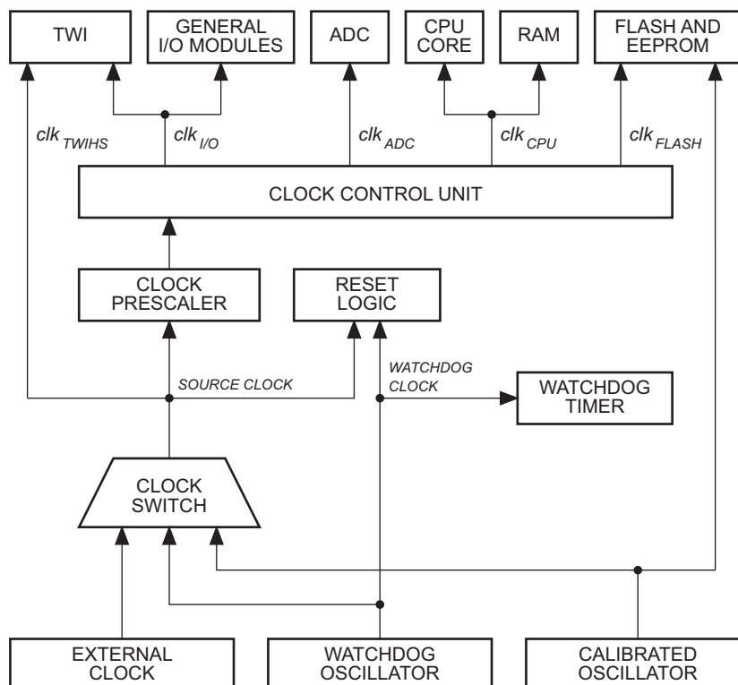
Figure 6-1. Clock Distribution
