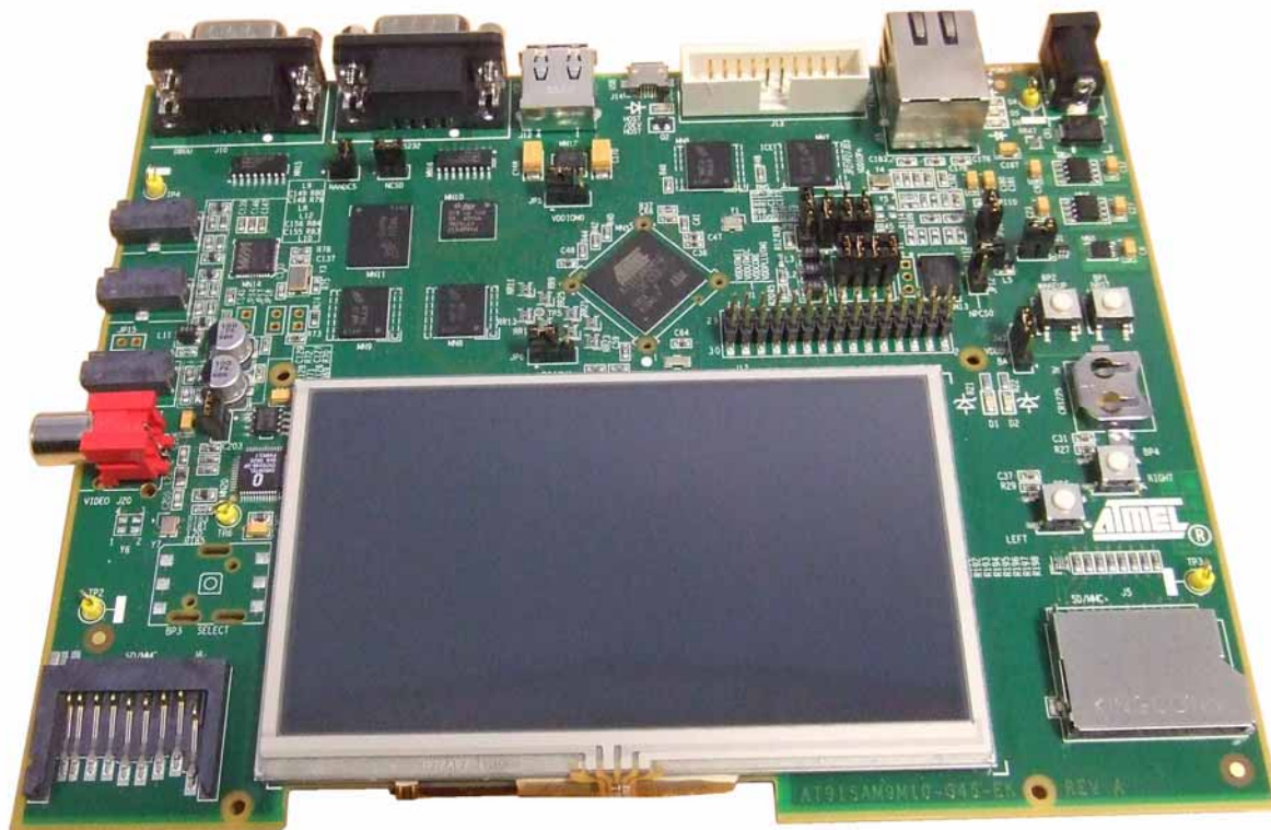
Figure 1-1. Board Photo
