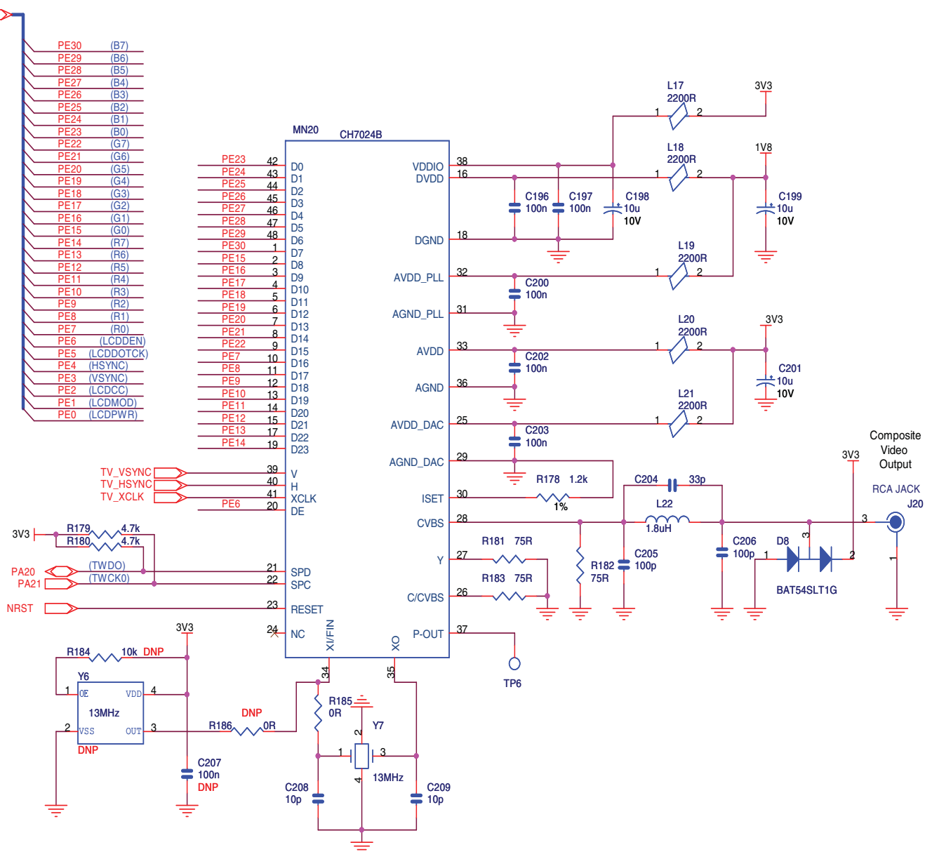
Figure 4-13. TV-Out Extension Port
