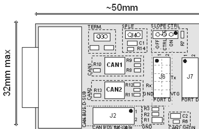
Figure 2. Component Placement
