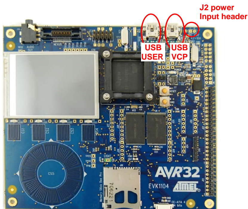
Figure 2-1 Possible power input interfaces on the EVK1104AU
