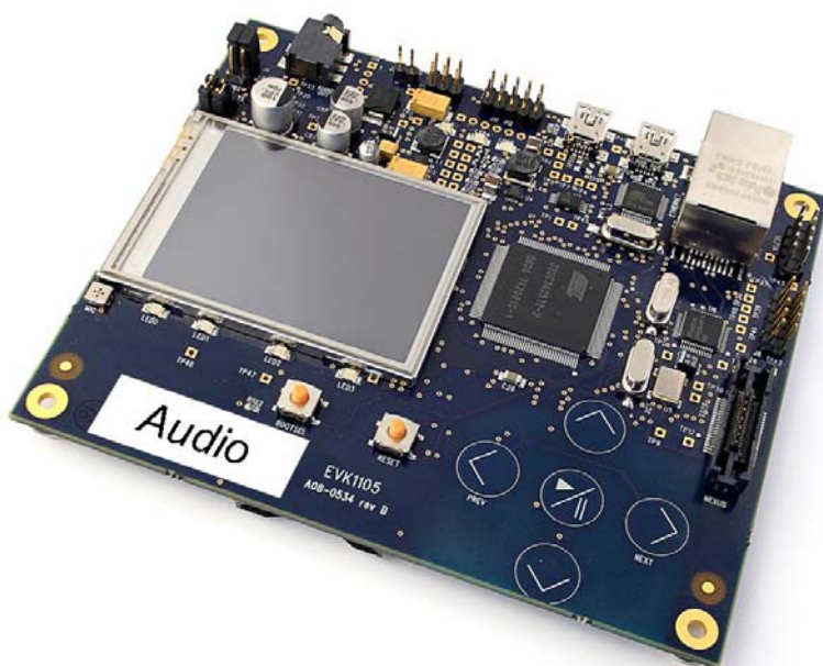
Figure 1-1 EVK1105AU board
