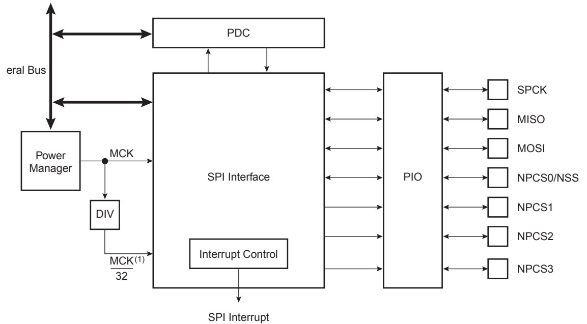
Figure 23-1. Block Diagram
