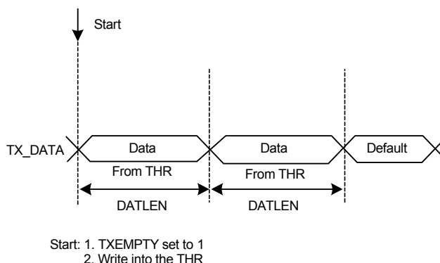
Figure 25-14. Transmit Frame Format in Continuous Mode
