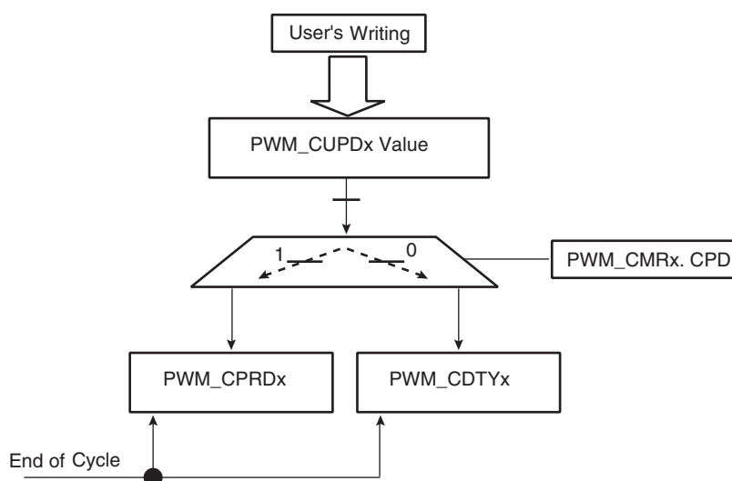
Figure 34-6. Synchronized Period or Duty Cycle Update
