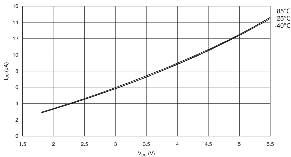
Figure 29-53. Watchdog Timer Current vs. V_{CC}
