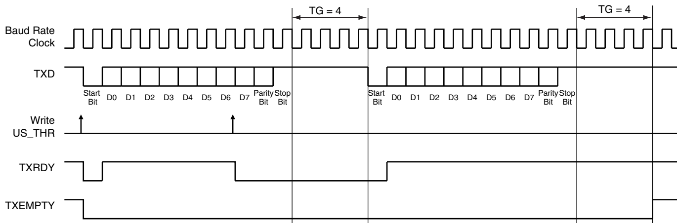
Figure 30-12. Timeguard Operations
