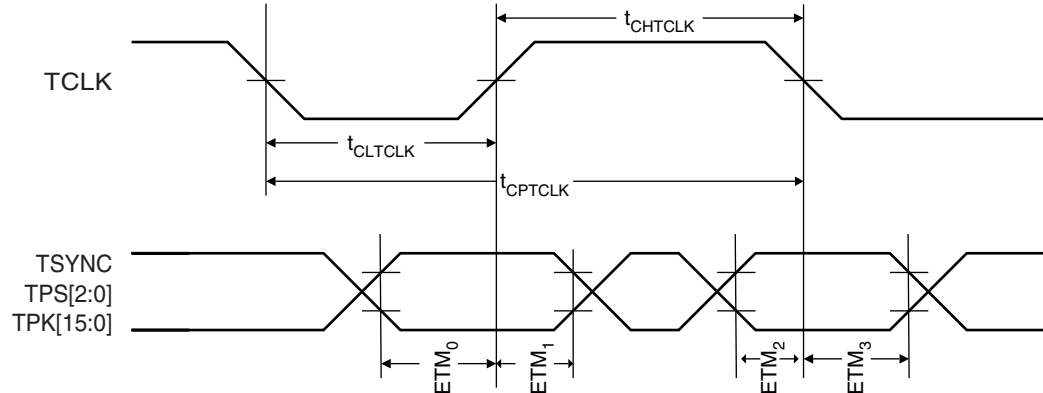
Figure 38-11. ETM Signals
