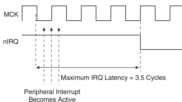
Figure 22-9. Internal Interrupt Level Sensitive Source
