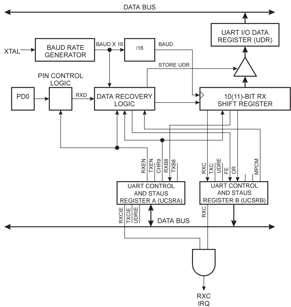
Figure 41. UART Receiver
