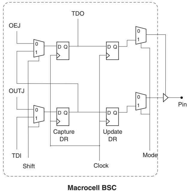
Macrocell BSC
