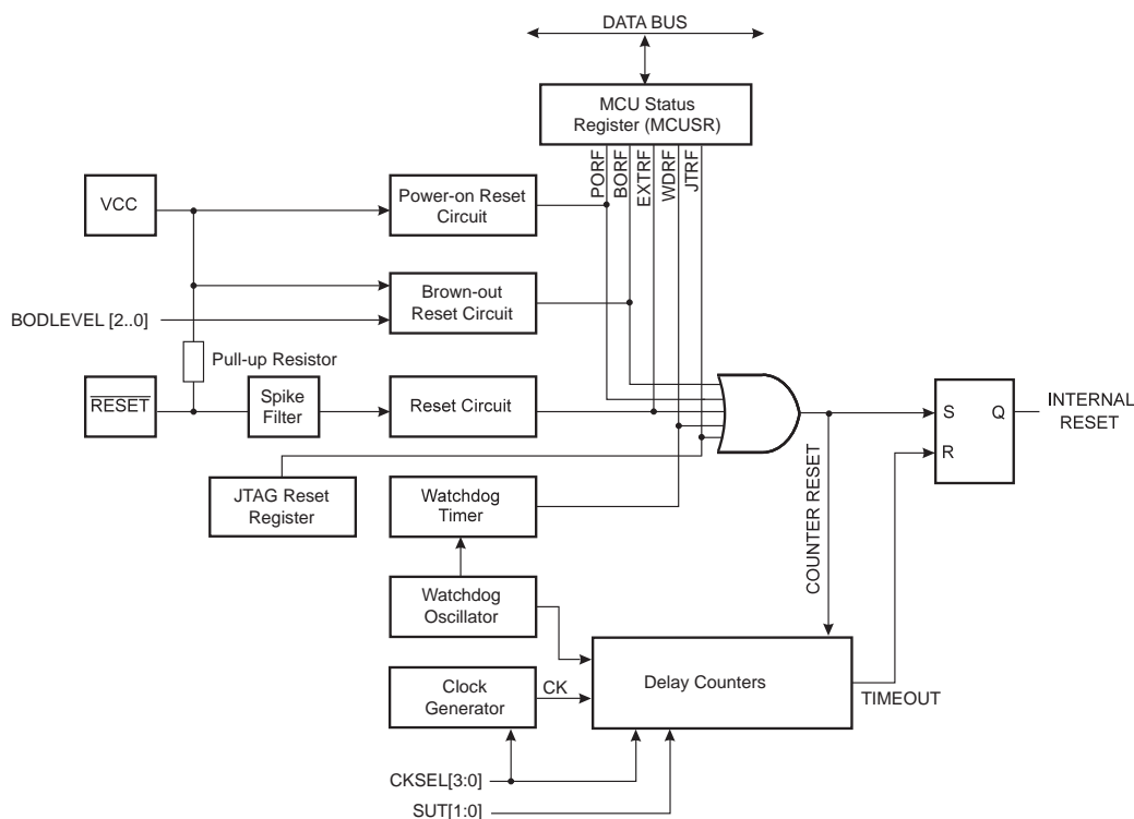
Figure 7-1. Reset Logic
