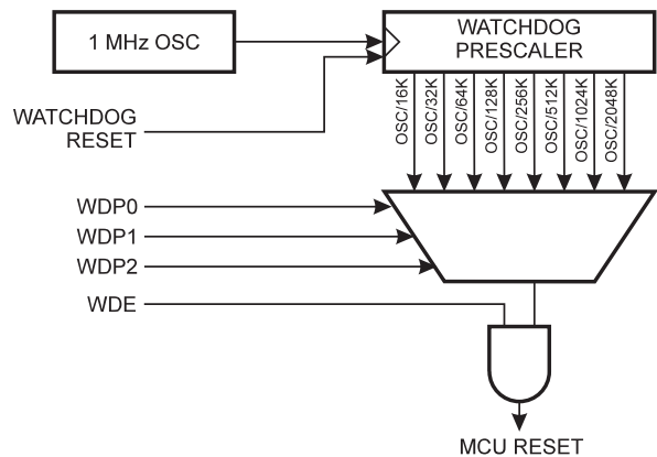
Figure 35. Watchdog Timer
