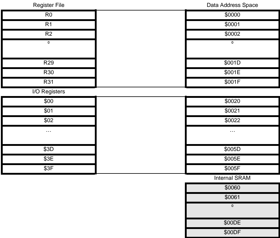
Figure 9. SRAM Organization
