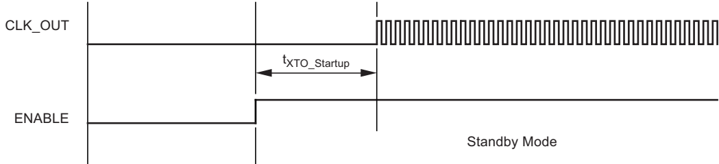
Figure 5-2. Standby Mode (CLK_OUT_CTRL0 or CLK_OUT_CTRL1 = 1)
