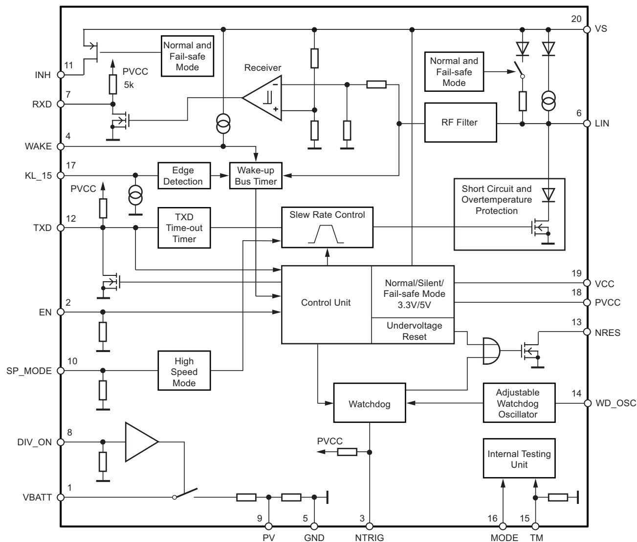
Figure 1-1. Block Diagram
