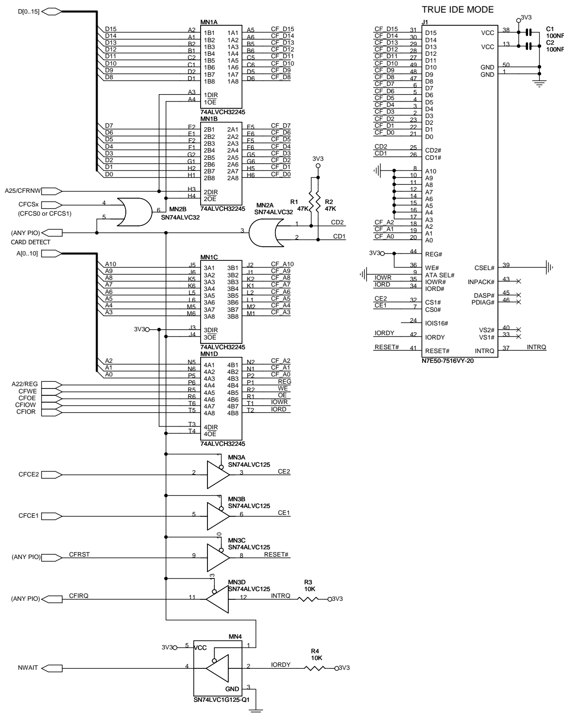
Figure 19-9. Hardware Configuration
