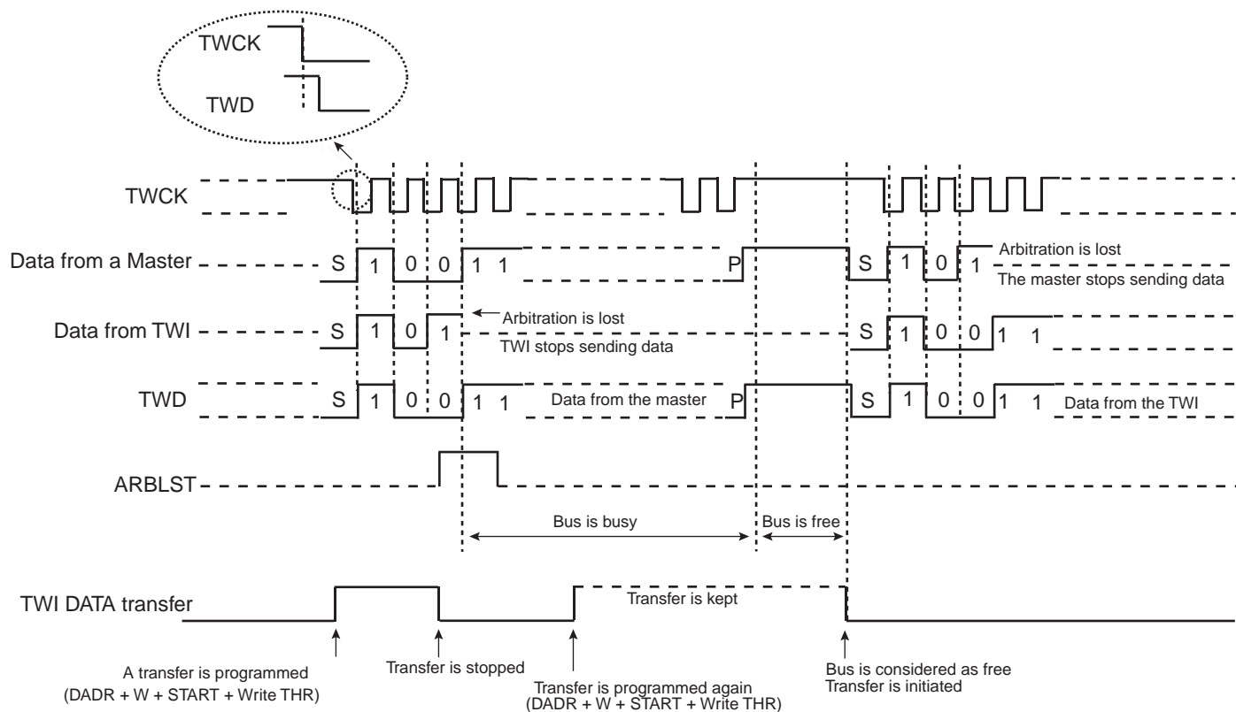
Figure 30-22. Arbitration Cases
