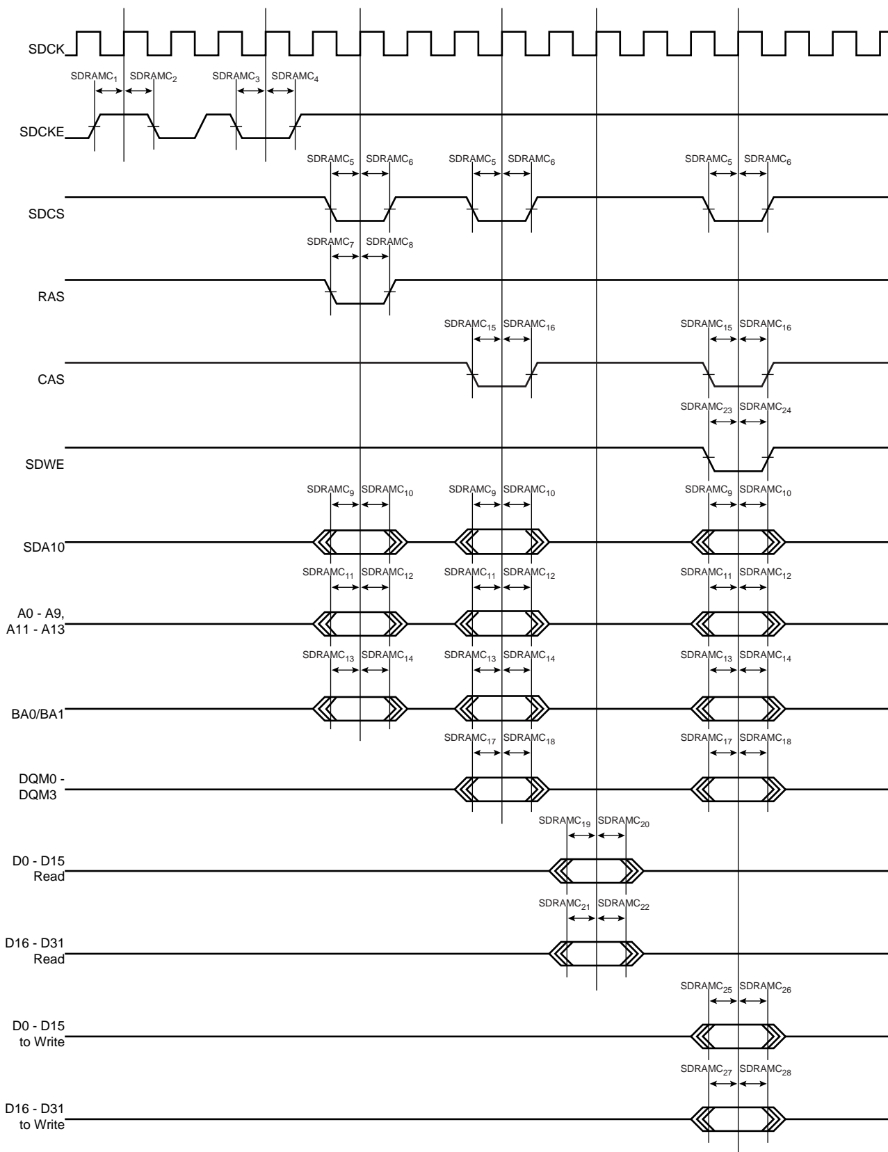
Figure 38-6. SDRAM Signals Relative to SDCK
