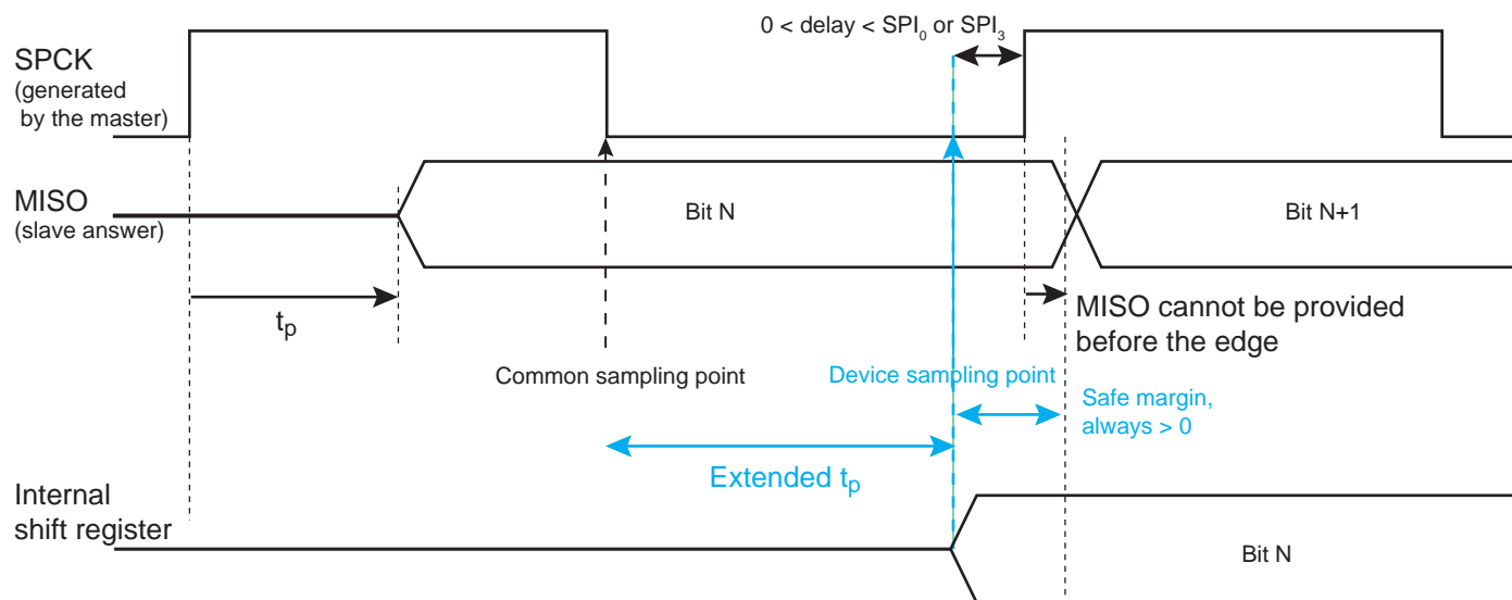
Figure 38-7. MISO Capture in Master Mode
