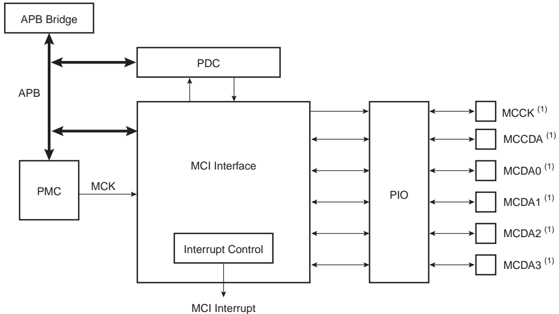
Figure 34-1. Block Diagram
