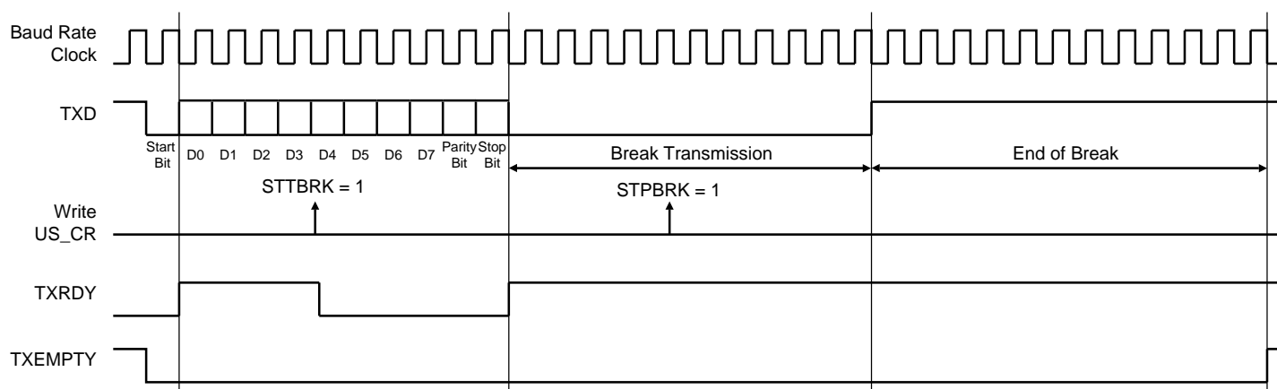
Figure 31-16. Break Transmission
