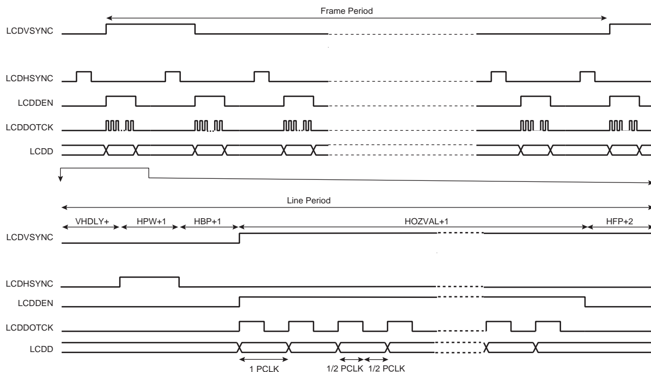
Figure 37-3. STN Panel Timing, CLKMOD 0
