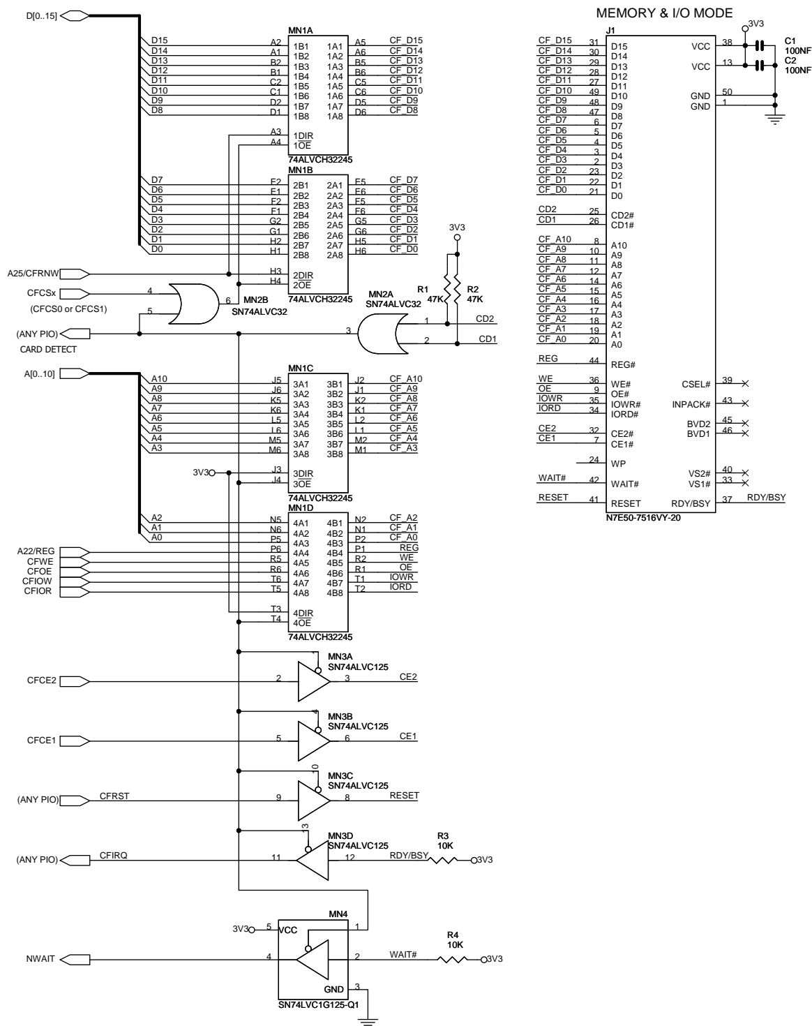
Figure 19-8. Hardware Configuration
