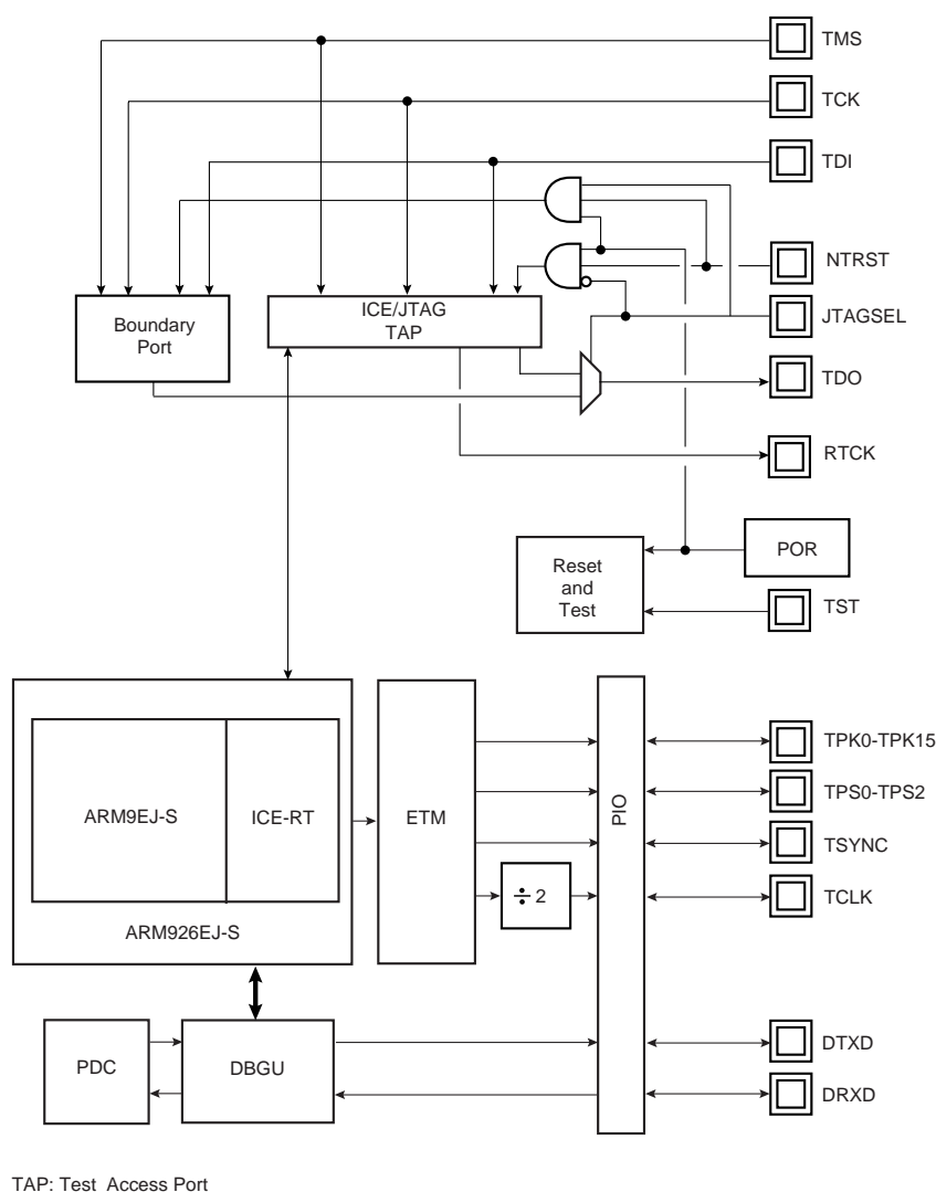
Figure 11-1. Debug and Test Block Diagram
