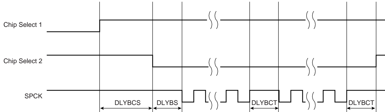
Figure 29-7. Programmable Delays
