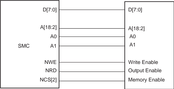
Figure 20-4. Memory Connection for a 16-bit Data Bus
