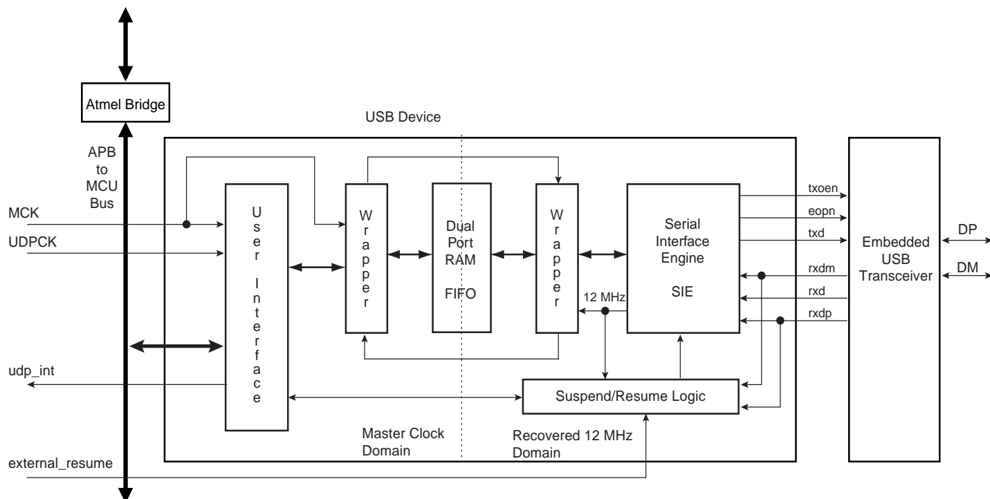
Figure 36-1. Block Diagram
