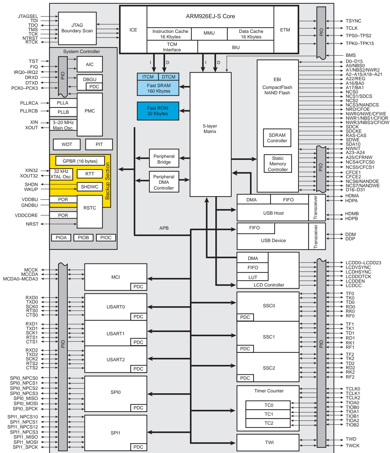
Figure 1-1. SAM9261 Block Diagram
