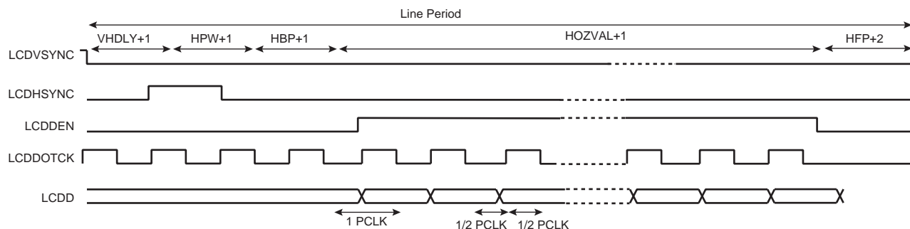
Figure 37-5. TFT Panel Timing (Line Expanded View), CLKMOD=1
