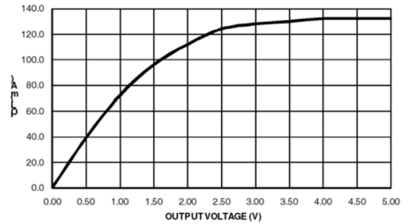
OUTPUT SINK CURRENT VS. OUTPUT VOLTAGE ( V_{CC} = 5V , T_A = 25^\circ\text{C} )
