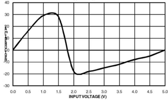
INPUT CURRENT VS. INPUT VOLTAGE ( V_{CC} = 5V , T_A = 25^\circ\text{C} )
