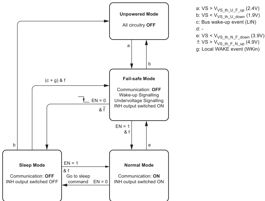
Figure 4-1. Operating Modes
