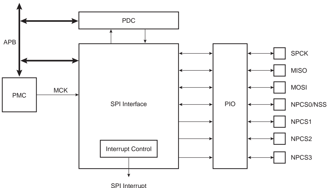
Figure 31-1. Block Diagram
