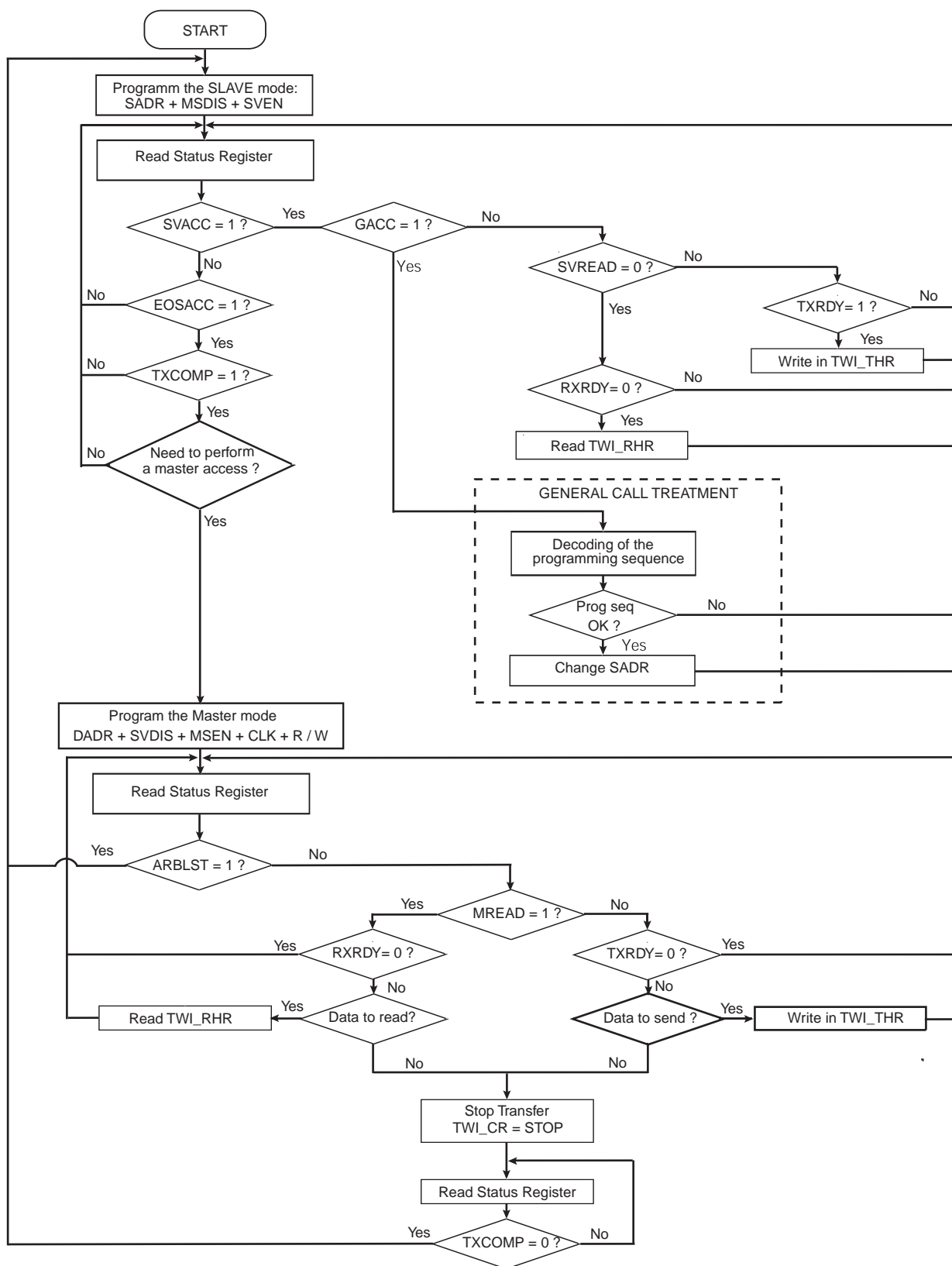
Figure 32-23. Multi-master Flowchart
