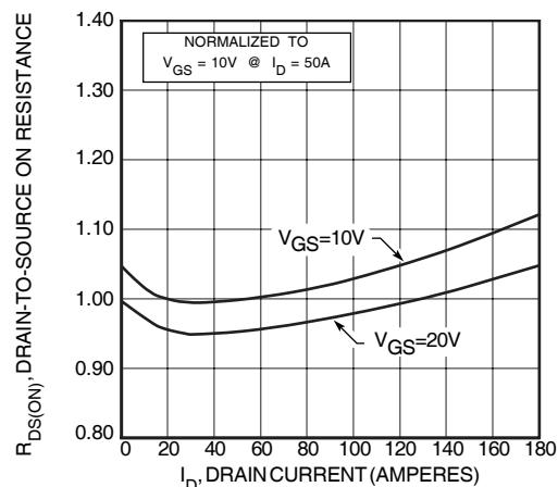
FIGURE 5, R_{\text{DS(ON)}} vs DRAIN CURRENT
