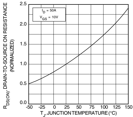
FIGURE 8, R_{\text{DS(ON)}} vs. TEMPERATURE
