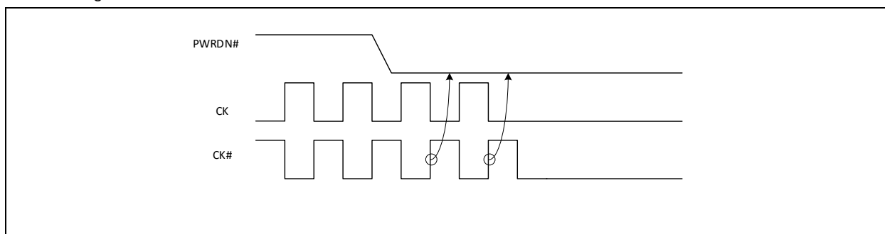
Figure 8. PWRDN# Assertion
