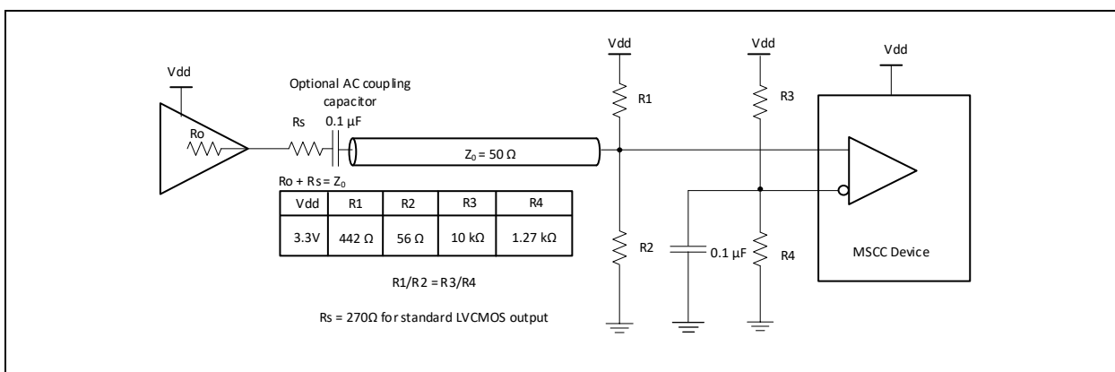
Figure 5. Input driven by a single ended output
