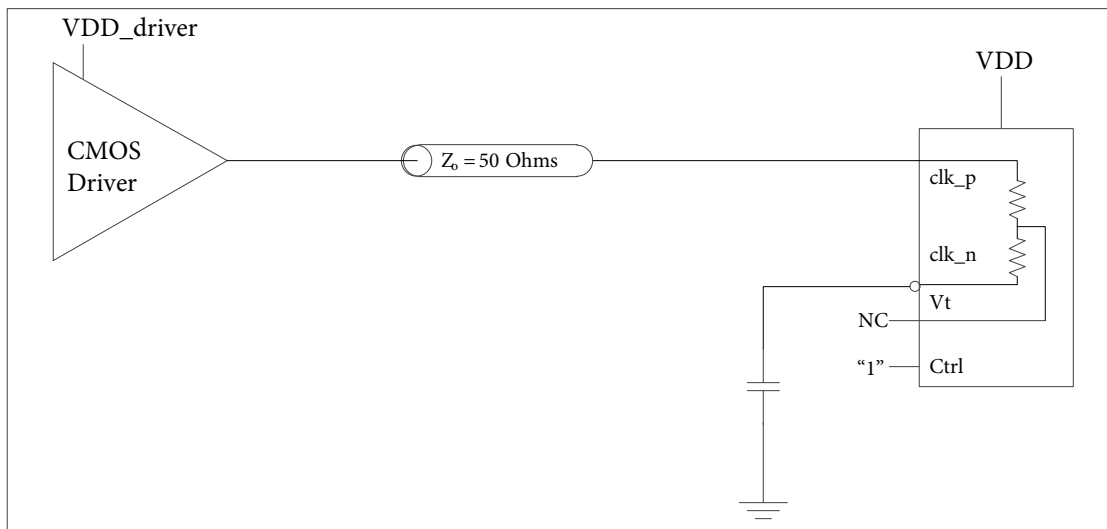
Figure 12 - Clock Input - DC-coupled 3.3V CMOS
