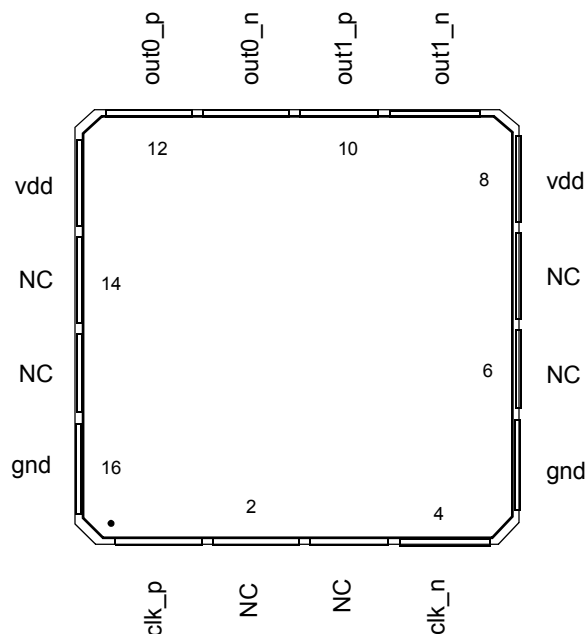
Figure 2 - Pin Connections
