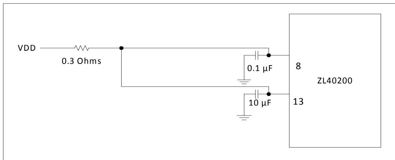
Figure 20 - Decoupling Connections for Power Pins
