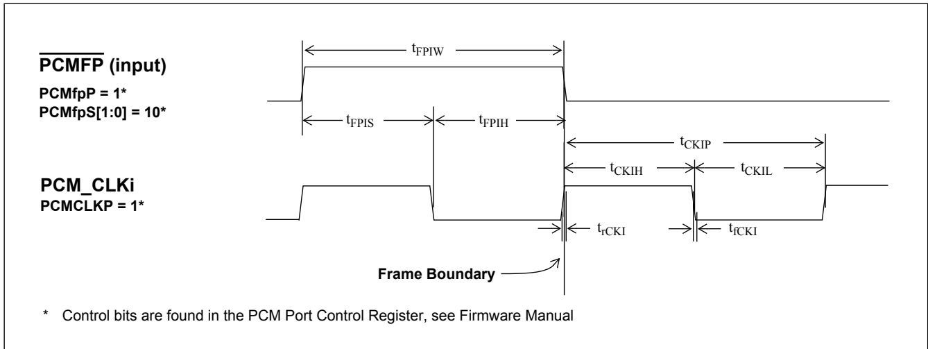
Figure 38 - TDM - McBSP \overline{\text{PCMFP}} and PCM_CLKi Input Timing
