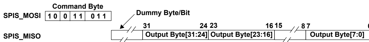
Figure 64 - SSPI Read Register Address 02A1 H
