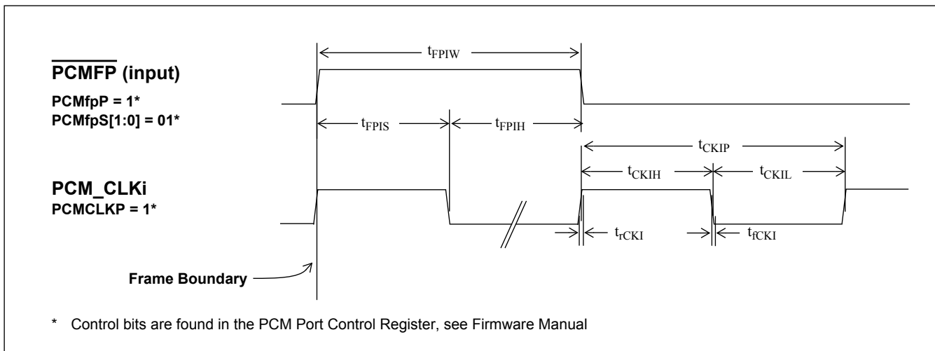
Figure 37 - TDM - GCI \overline{\text{PCMFP}} and PCM_CLKi Input Timing
