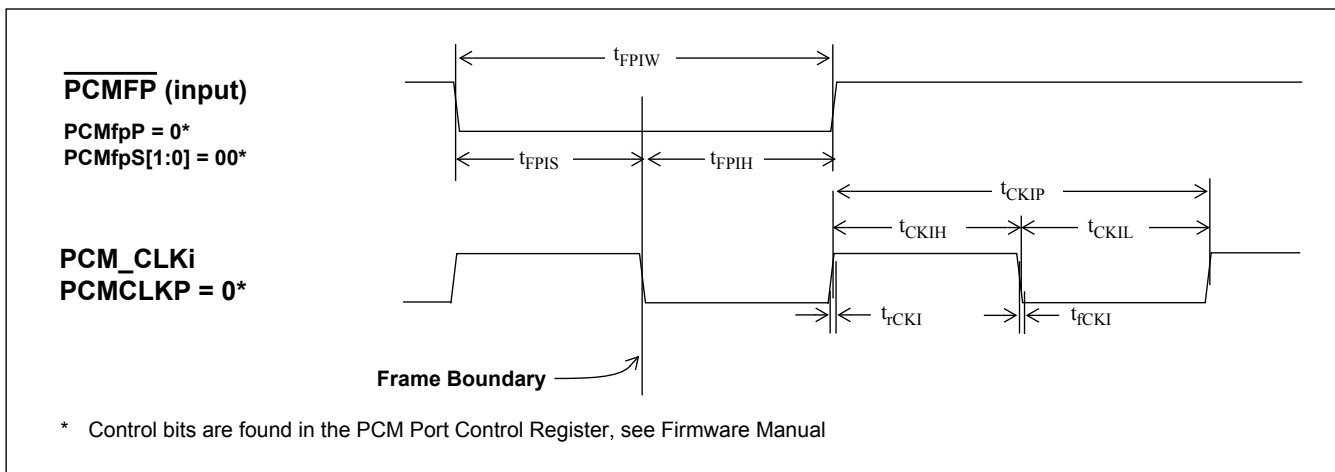
Figure 36 - TDM - ST-BUS \overline{\text{PCMFP}} and PCM_CLKi Input Timing
