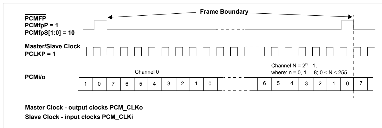
Figure 14 - TDM - McBSP Slave/Master Functional Timing Diagram
