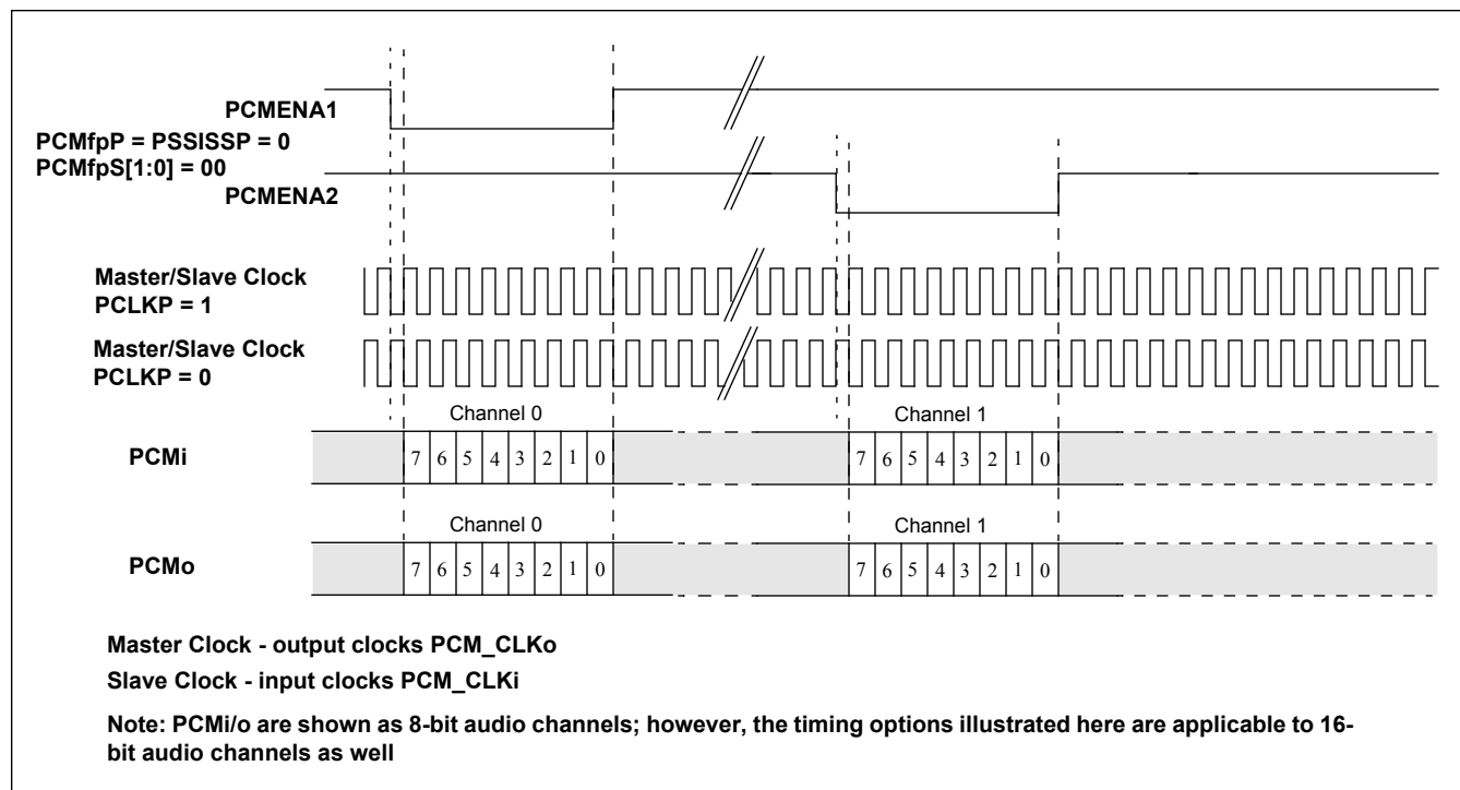
Figure 16 - SSI Mode: Separated Channels Functional Timing
