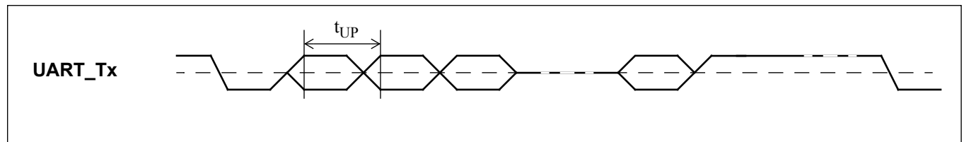
Figure 53 - UART_Tx Timing
