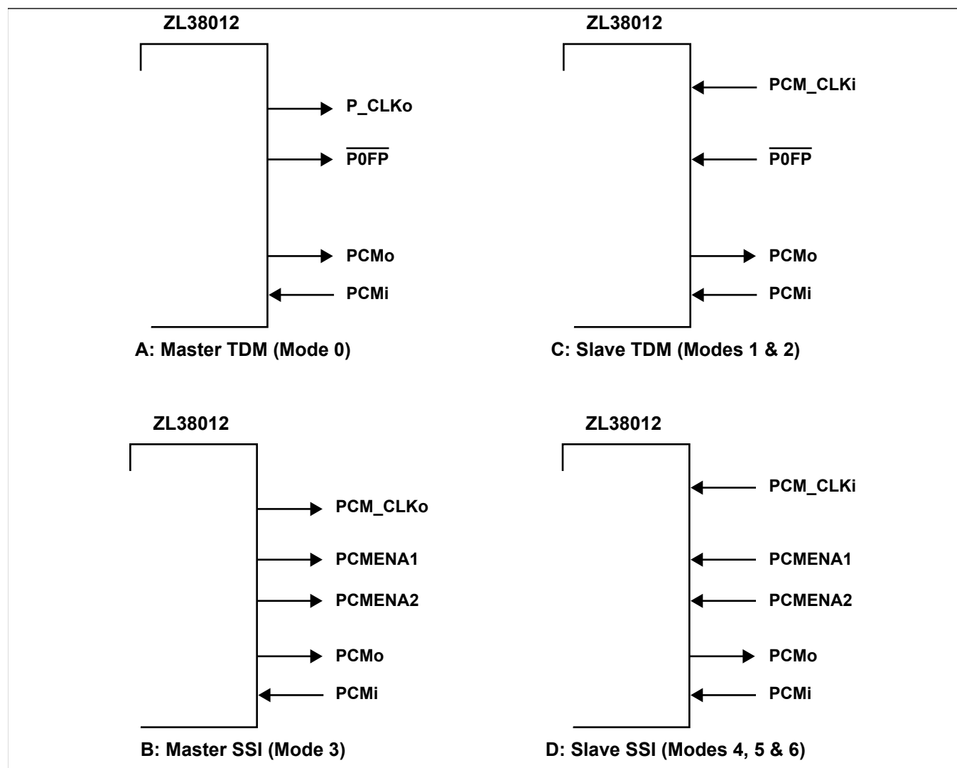
Figure 5 - PCM Port Signal Configurations for Master/Slave Operation
