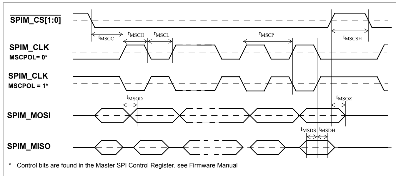
Figure 48 - Master SPI Timing (MSCPHA = 1)
