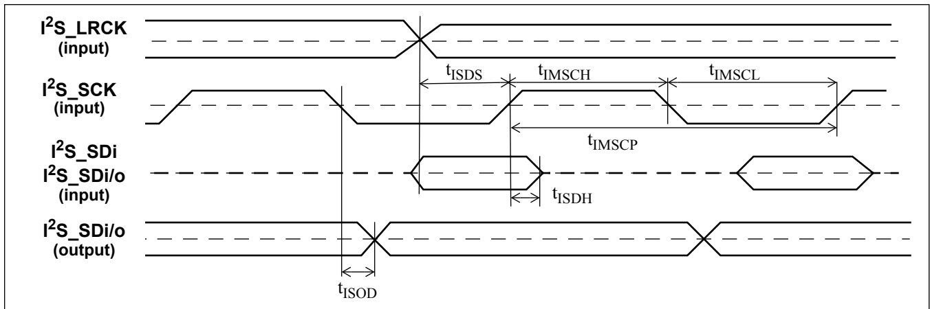
Figure 49 - Slave I 2 S Timing
