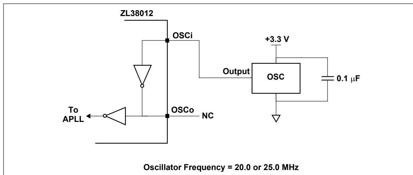
Figure 57 - Crystal Oscillator Application Circuit
