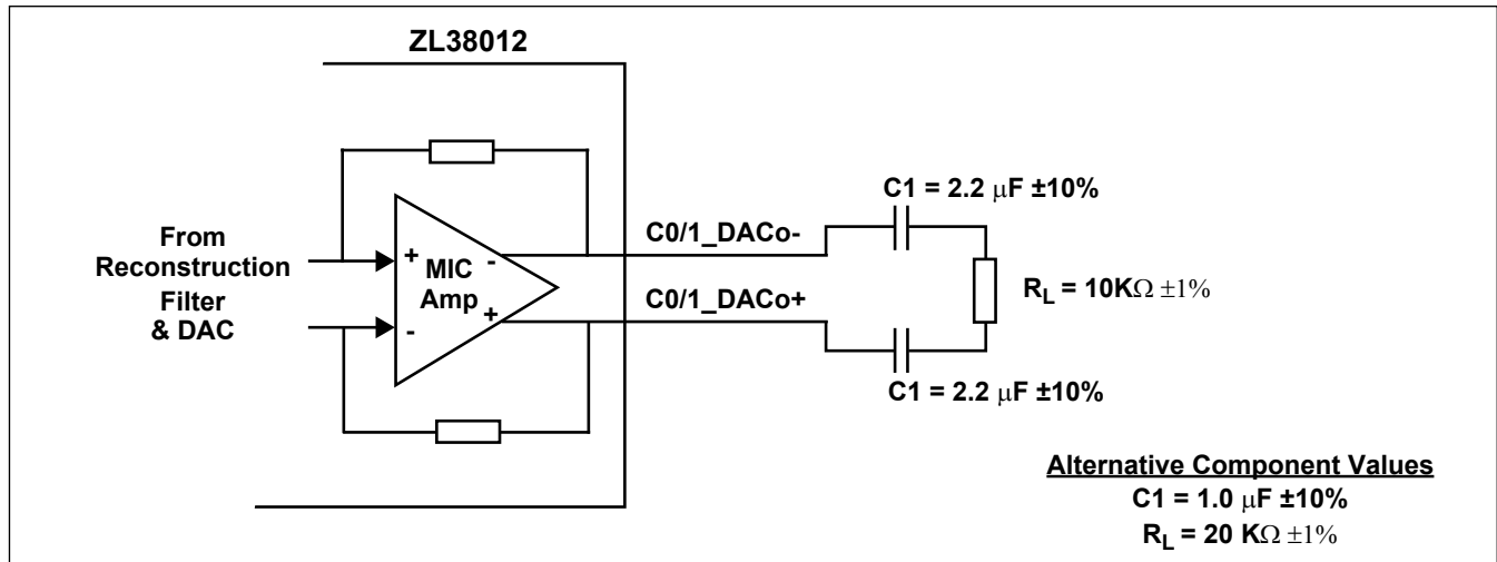
Figure 60 - CODEC 0/1 DAC Differential Driver Circuit
