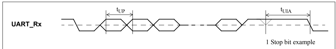
Figure 52 - UART_Rx Timing
