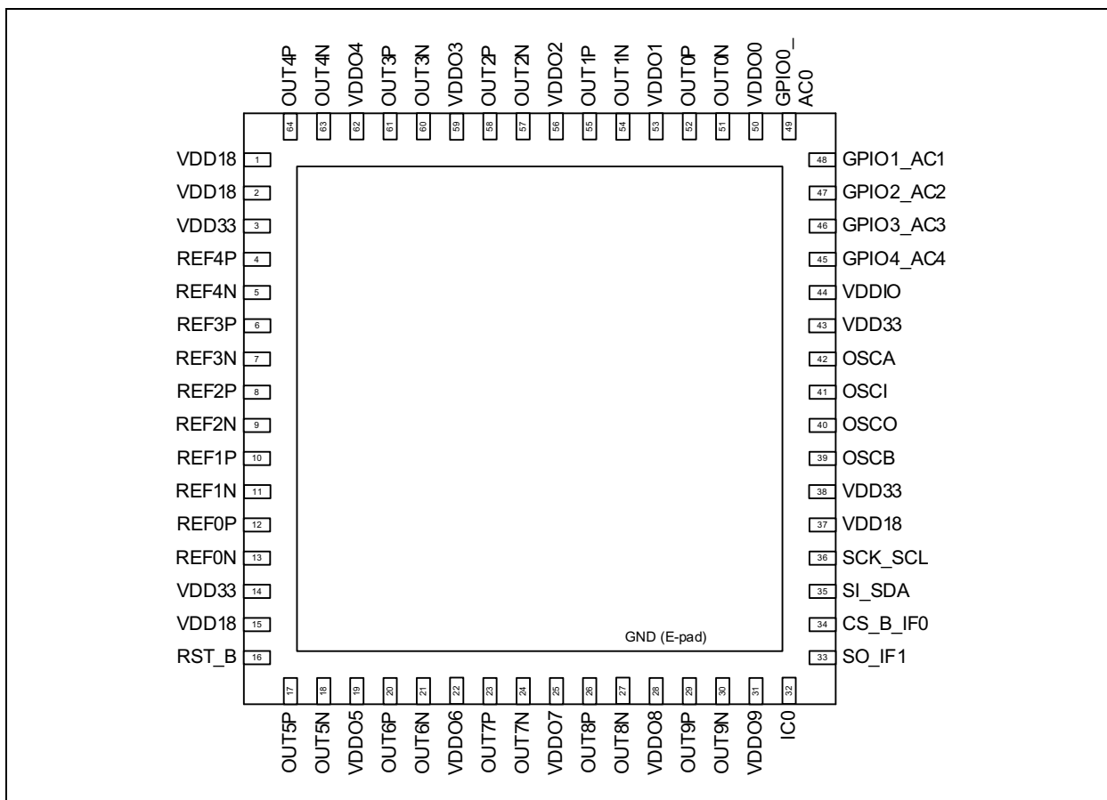
FIGURE 1: 64-Lead 9 mm x 9 mm VQFN (0.5 mm pitch) for ZL30641, ZL30642, ZL30643, ZL30644, ZL30645.
