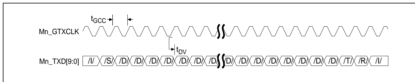
Figure 55 - TBI Transmit Timing Diagram
