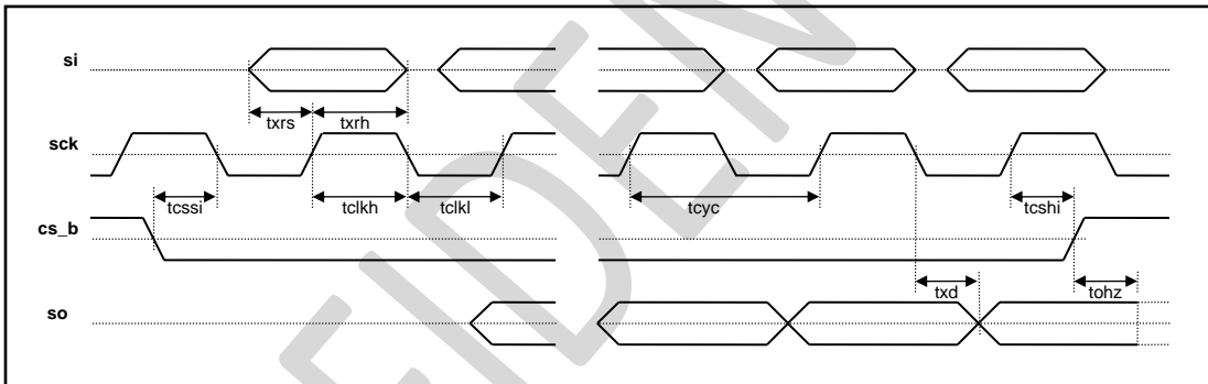
Figure 31 - SPI Slave Interface Timing, LSB First Mode
