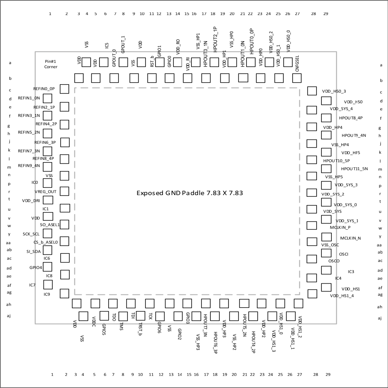
FIGURE 4-1: Pin Diagram.
