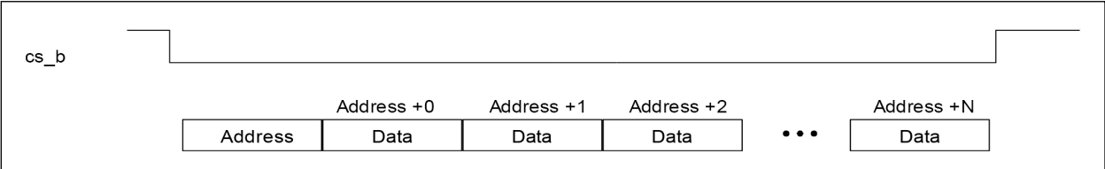
FIGURE 8-4: Example of the Burst Mode Operation.
