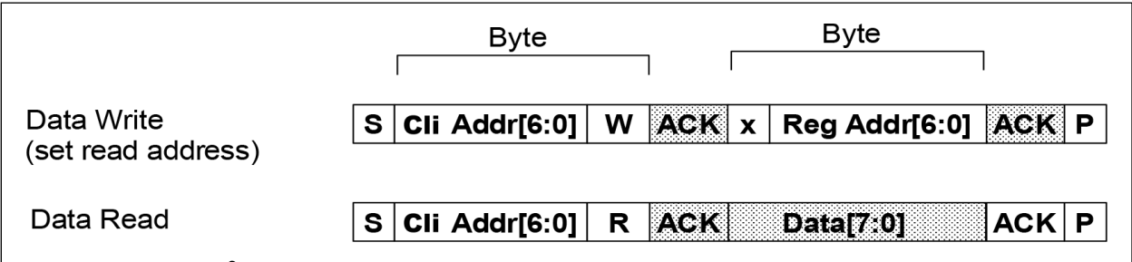
FIGURE 8-6: I 2 C Data Read Protocol.
