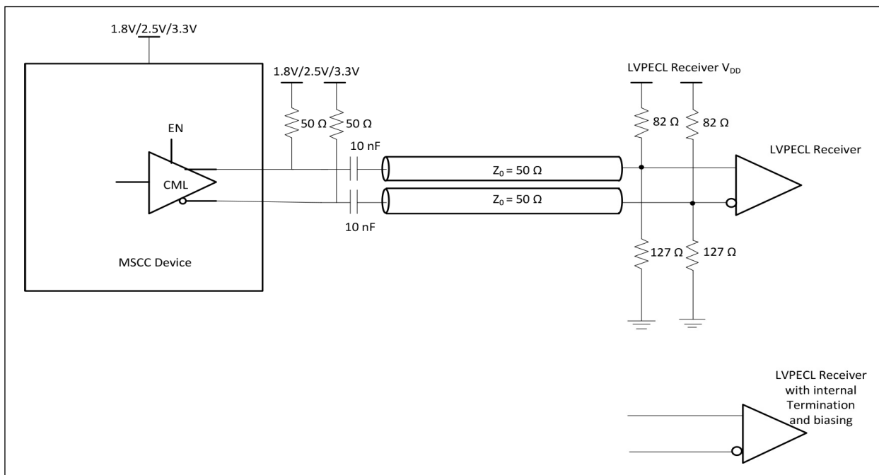
FIGURE 6-14: Driving LVPECL Receiver.
