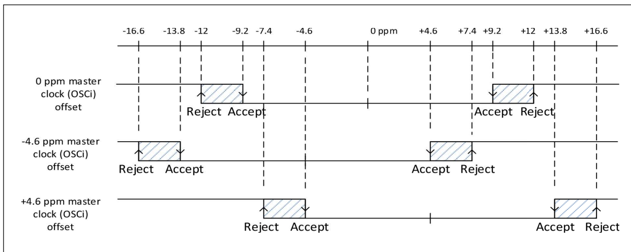
FIGURE 6-1: Stratum 3/G.8262 Option I Frequency Acceptance and Rejection Ranges.
