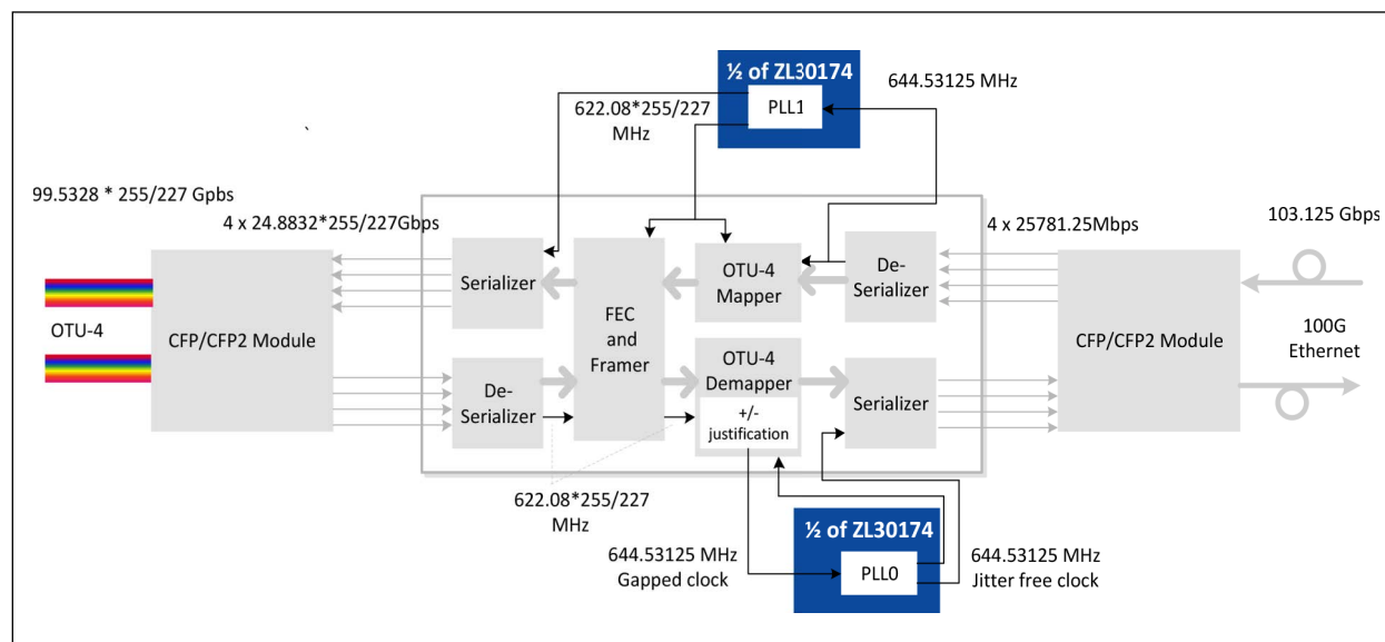
FIGURE 3-1: OTU-4 Transponder.
