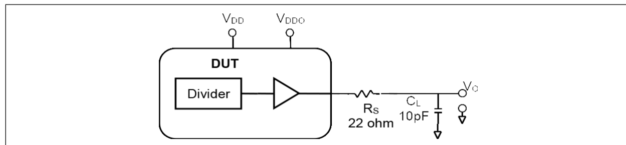
FIGURE 10-2: HPOUT and GPOUT (CMOS) Output.
