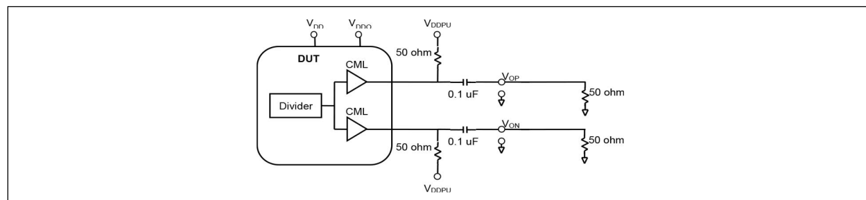
FIGURE 10-1: HPOUT_DIFF (CML) Output.
