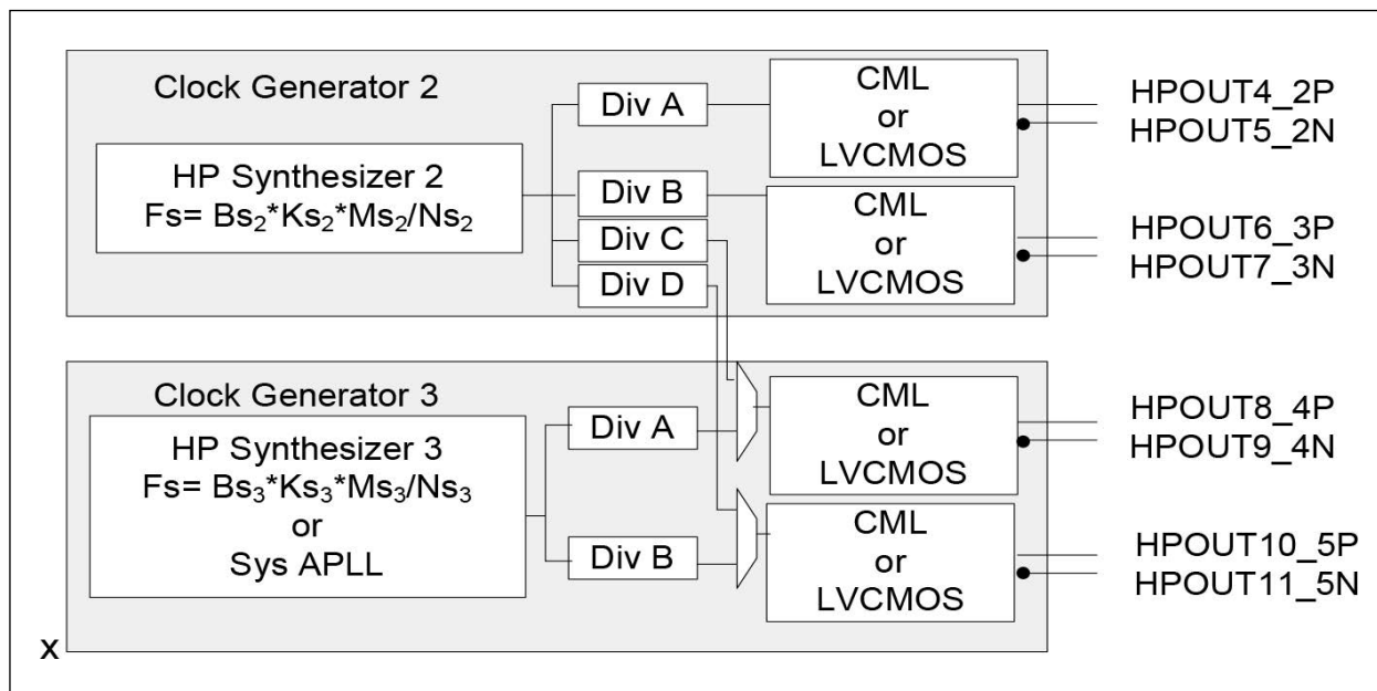
FIGURE 6-18: HPOUT[8:9] MUX.
