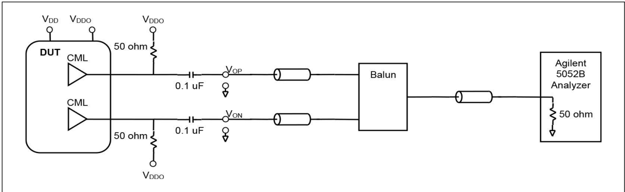
FIGURE 11-1: HPOUT_DIFF (CML) Output Jitter Test Circuit.
