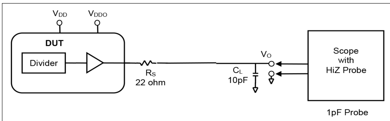
FIGURE 10-11: HPOUT and GPOUT Output t_r , t_f , and Duty Cycle Measurement Setup.
