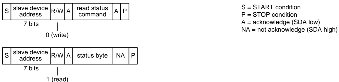
Figure 18 – I 2 C EEPROM Read Status Transaction Functional Timing
