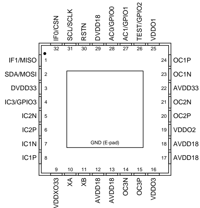
Figure 4 - Pin Diagram
