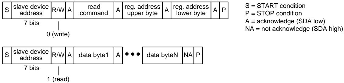
Figure 15 – I 2 C Read Transaction Functional Timing
