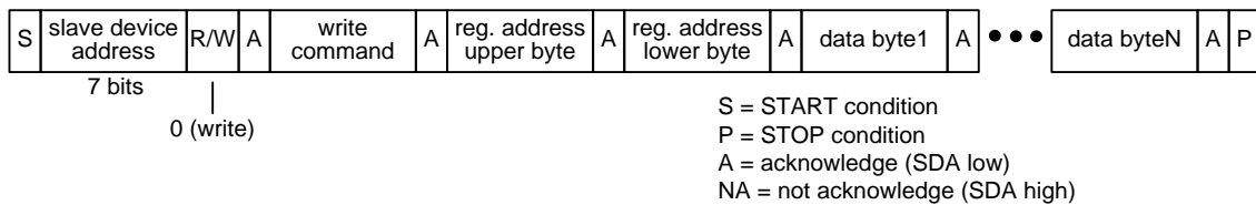
Figure 16 – I 2 C Register Write Transaction Functional Timing
