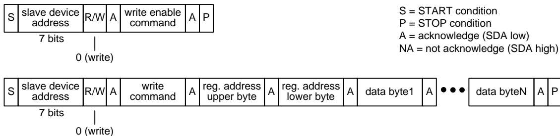
Figure 17 – I 2 C EEPROM Write Transaction Functional Timing
