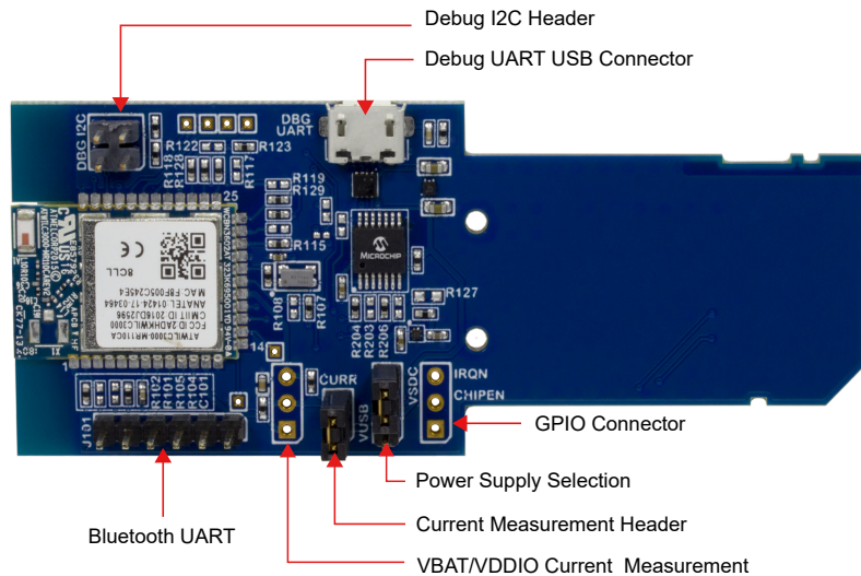
Figure 1-1. WILC3000 SD Interfaces
