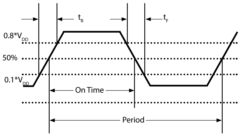
Fig 2: Output Waveform
