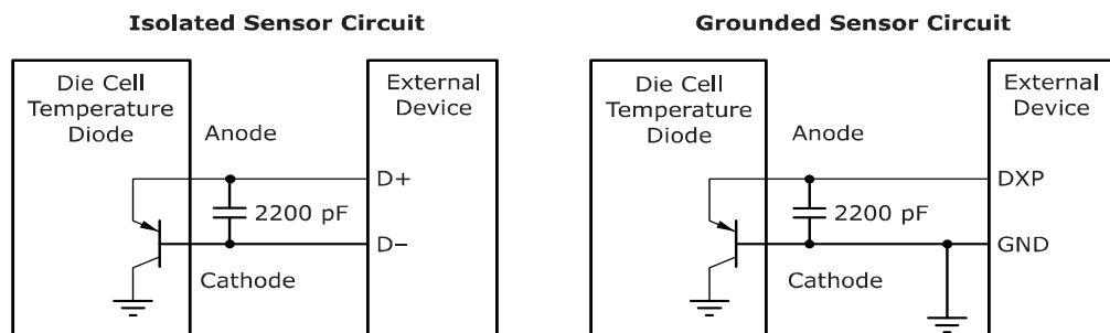
FIGURE 8-1: THERMAL DIODE
